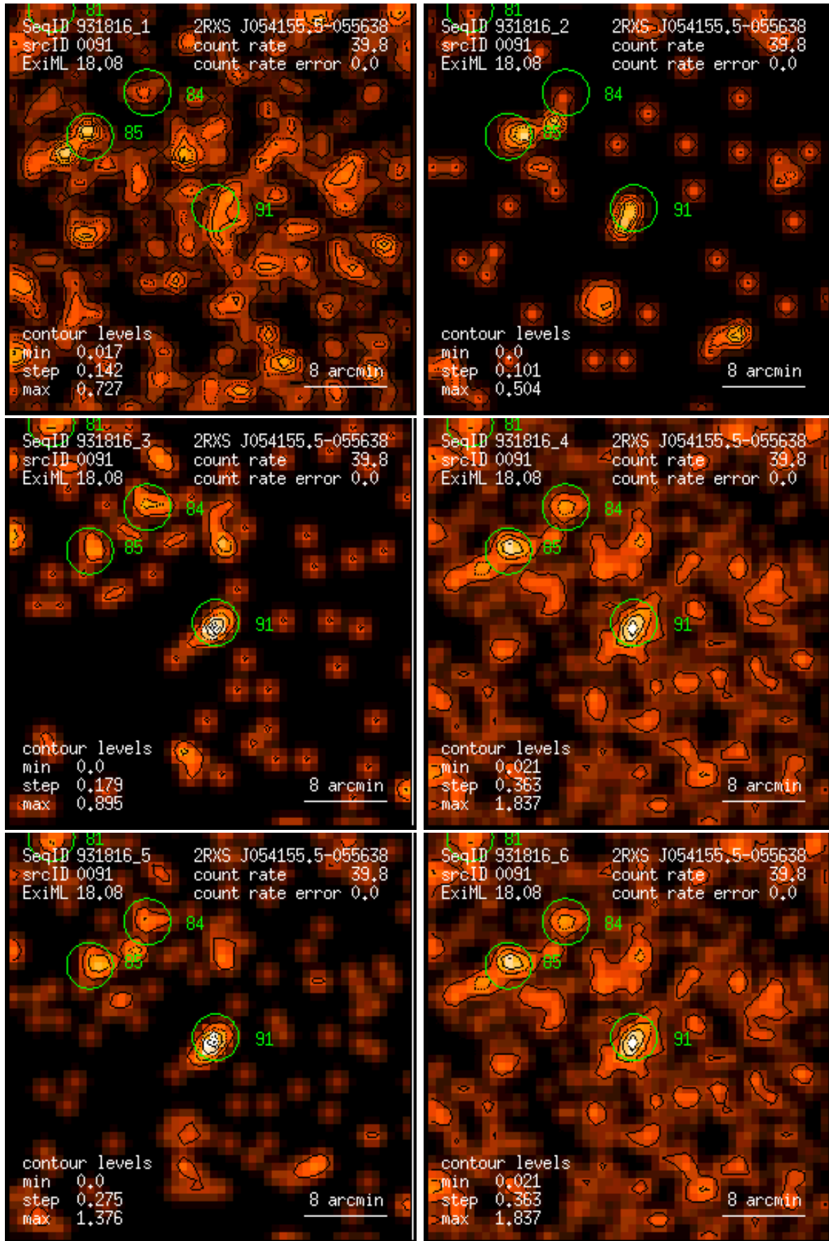
Figure 91: RASS 931816: detection 0091: band rate images, Gaussian filter: (1) PSPC channels 11 – 41, (2) 52 – 90, (3) 91 – 201, (4) 11 – 235, (5) 52 – 201, (6) 11 – 201. Broad band rates in counts/ks. Band rate contour levels in counts/ks/arcmin 2 .
