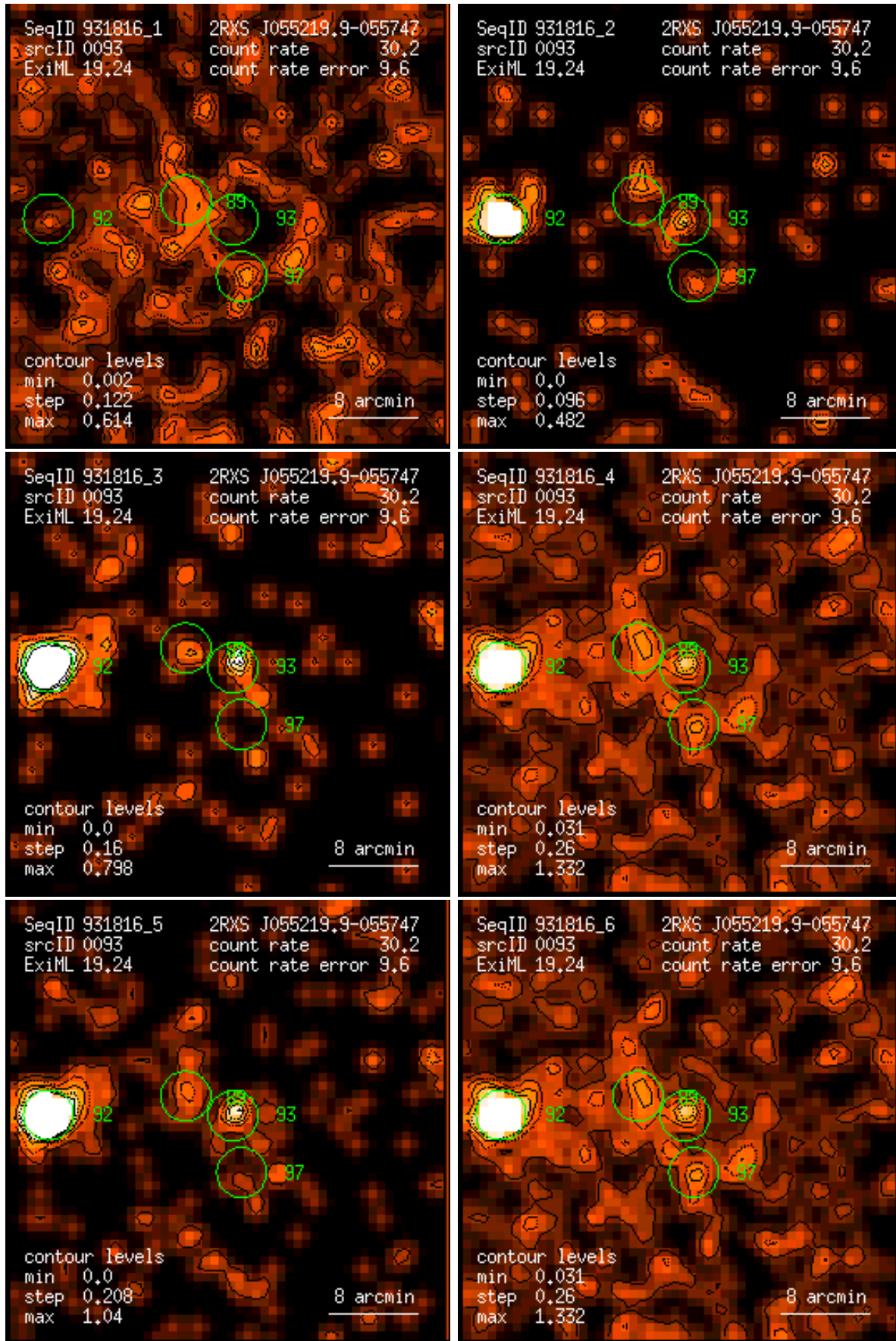
Figure 93: RASS 931816: detection 0093: band rate images, Gaussian filter: (1) PSPC channels 11 – 41, (2) 52 – 90, (3) 91 – 201, (4) 11 – 235, (5) 52 – 201, (6) 11 – 201. Broad band rates in counts/ks. Band rate contour levels in counts/ks/arcmin 2 .
