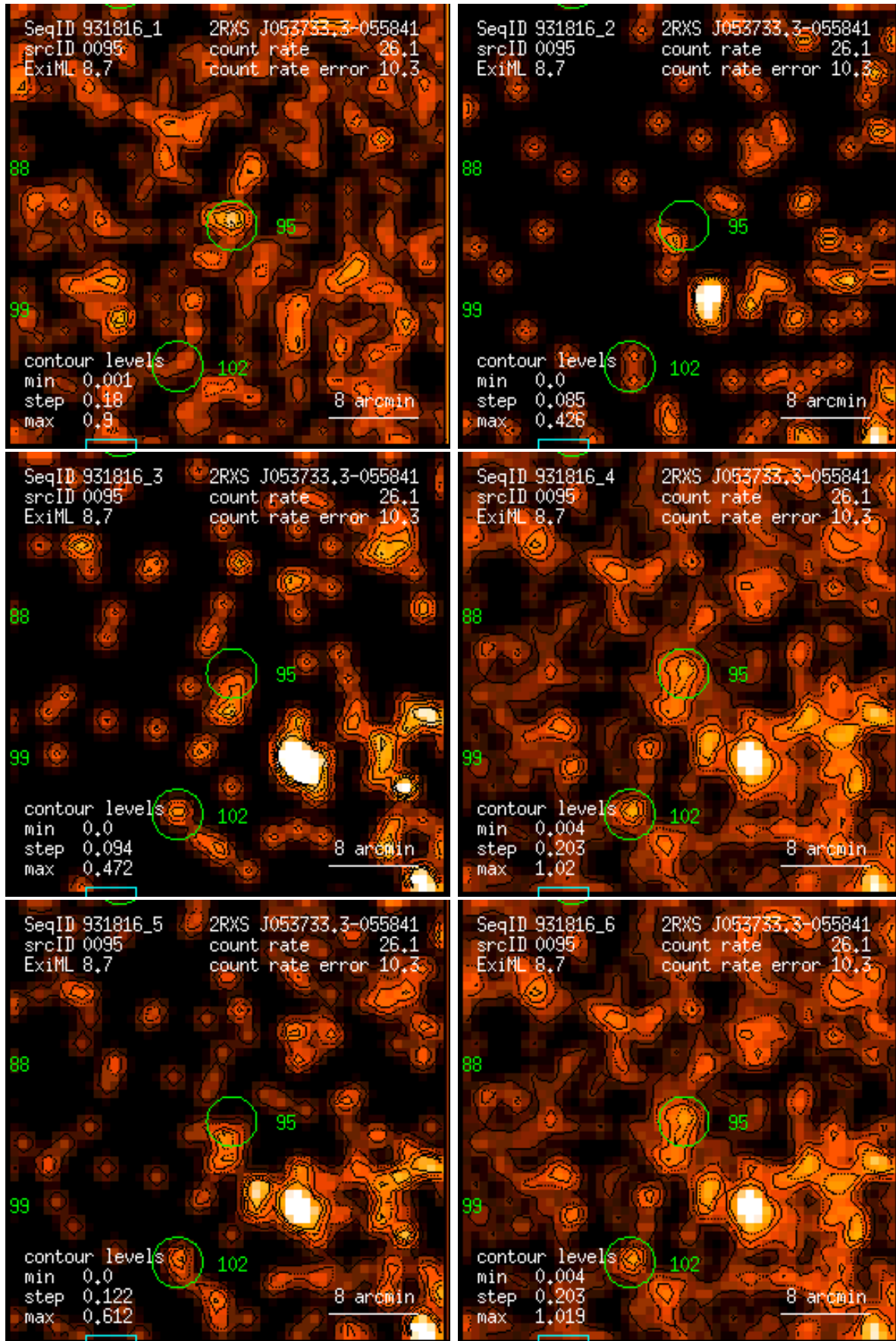
Figure 95: RASS 931816: detection 0095: band rate images, Gaussian filter: (1) PSPC channels 11 – 41, (2) 52 – 90, (3) 91 – 201, (4) 11 – 235, (5) 52 – 201, (6) 11 – 201. Broad band rates in counts/ks. Band rate contour levels in counts/ks/arcmin 2 .
