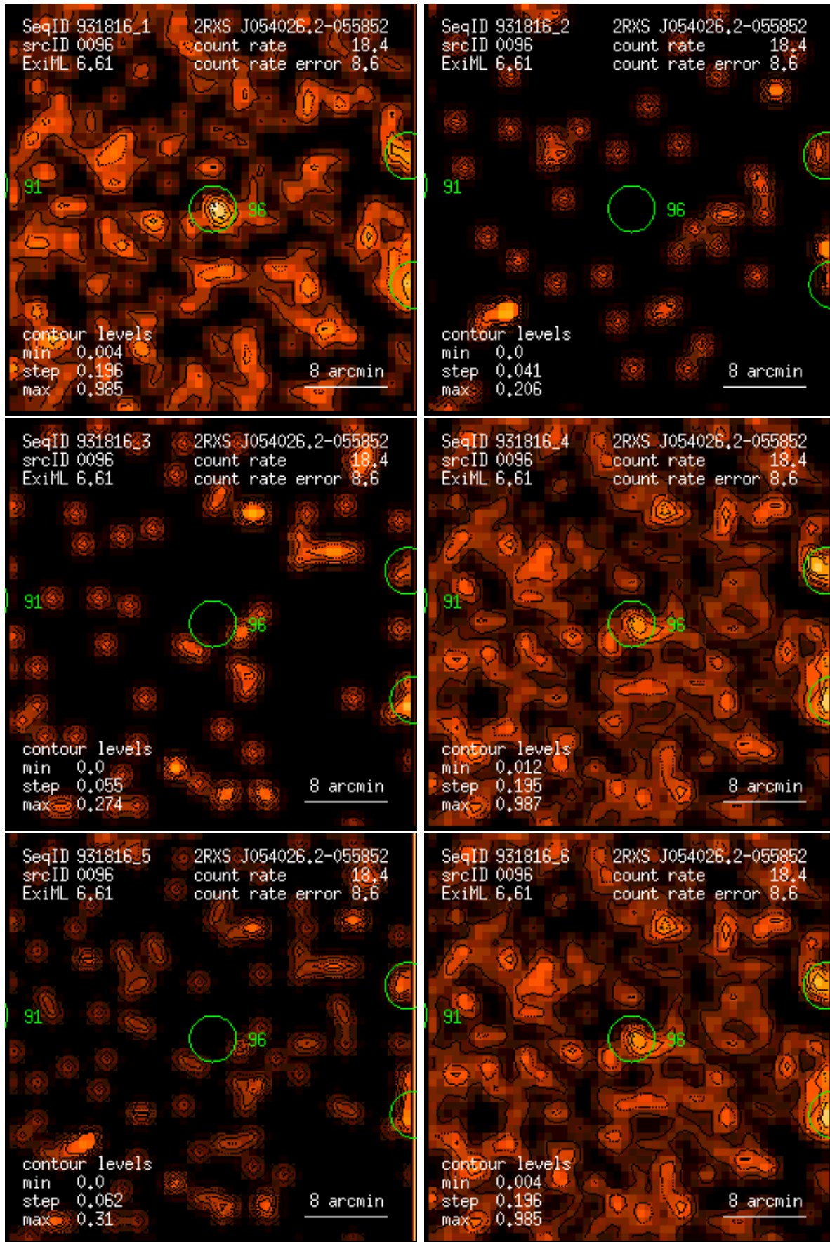
Figure 96: RASS 931816: detection 0096: band rate images, Gaussian filter: (1) PSPC channels 11 – 41, (2) 52 – 90, (3) 91 – 201, (4) 11 – 235, (5) 52 – 201, (6) 11 – 201. Broad band rates in counts/ks. Band rate contour levels in counts/ks/arcmin 2 .
