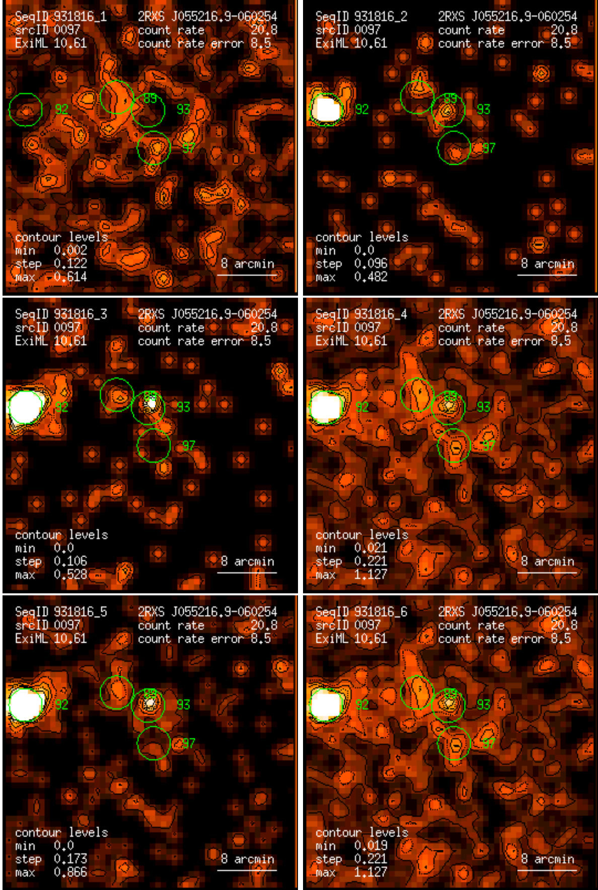
Figure 97: RASS 931816: detection 0097: band rate images, Gaussian filter: (1) PSPC channels 11 – 41, (2) 52 – 90, (3) 91 – 201, (4) 11 – 235, (5) 52 – 201, (6) 11 – 201. Broad band rates in counts/ks. Band rate contour levels in counts/ks/arcmin 2 .
