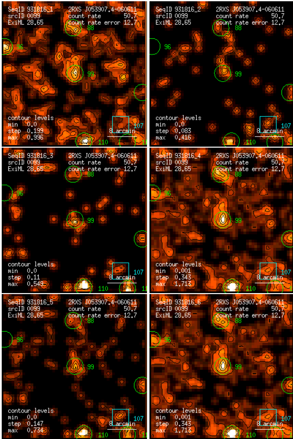
Figure 99: RASS 931816: detection 0099: band rate images, Gaussian filter: (1) PSPC channels 11 – 41, (2) 52 – 90, (3) 91 – 201, (4) 11 – 235, (5) 52 – 201, (6) 11 – 201. Broad band rates in counts/ks. Band rate contour levels in counts/ks/arcmin 2 .
