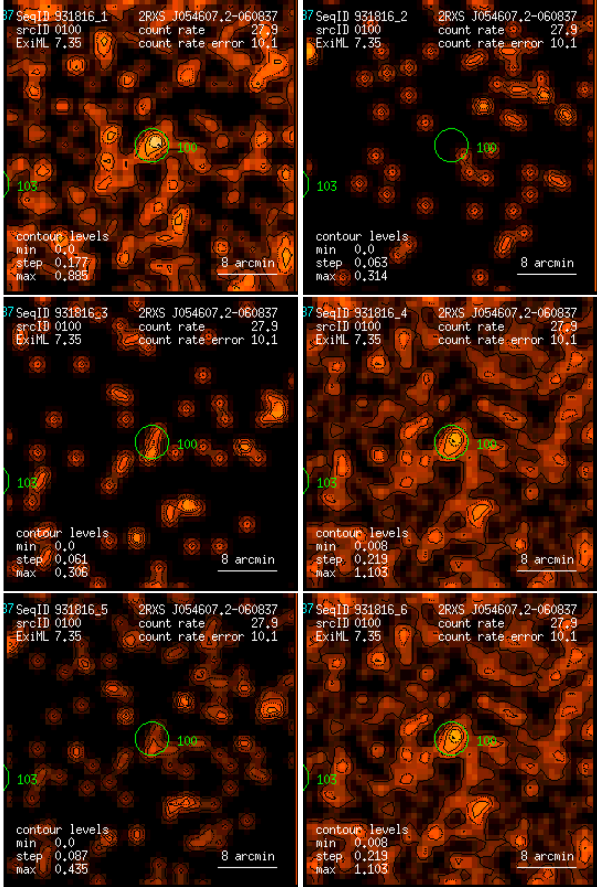
Figure 100: RASS 931816: detection 0100: band rate images, Gaussian filter: (1) PSPC channels 11 – 41, (2) 52 – 90, (3) 91 – 201, (4) 11 – 235, (5) 52 – 201, (6) 11 – 201. Broad band rates in counts/ks. Band rate contour levels in counts/ks/arcmin 2 .
