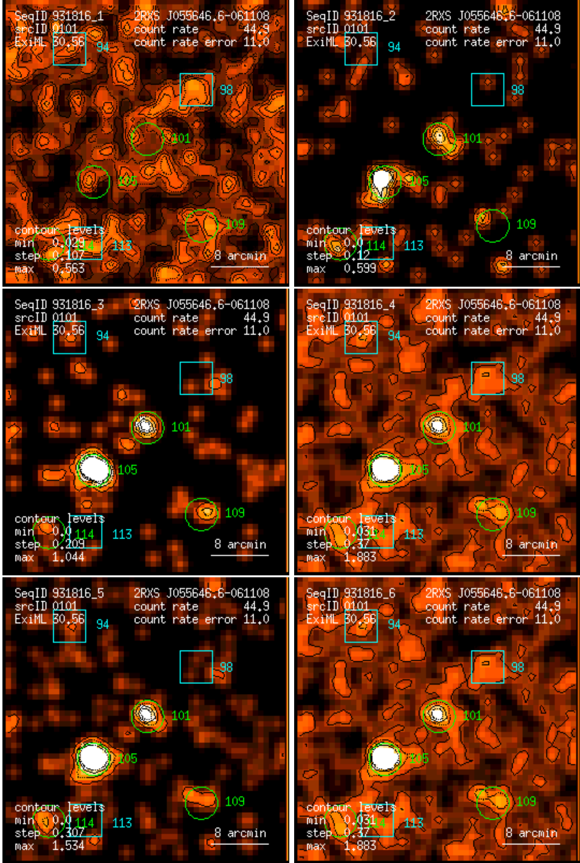
Figure 101: RASS 931816: detection 0101: band rate images, Gaussian filter: (1) PSPC channels 11 – 41, (2) 52 – 90, (3) 91 – 201, (4) 11 – 235, (5) 52 – 201, (6) 11 – 201. Broad band rates in counts/ks. Band rate contour levels in counts/ks/arcmin 2 .
