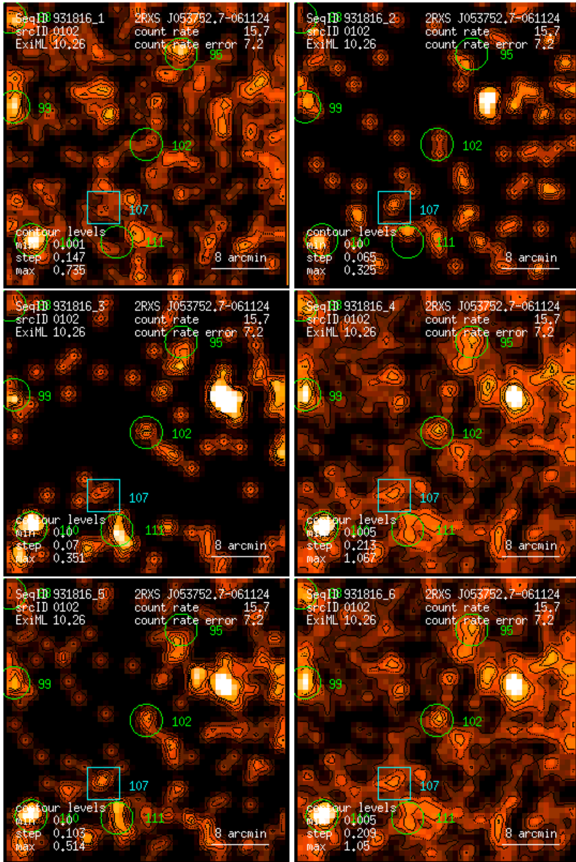
Figure 102: RASS 931816: detection 0102: band rate images, Gaussian filter: (1) PSPC channels 11 – 41, (2) 52 – 90, (3) 91 – 201, (4) 11 – 235, (5) 52 – 201, (6) 11 – 201. Broad band rates in counts/ks. Band rate contour levels in counts/ks/arcmin 2 .
