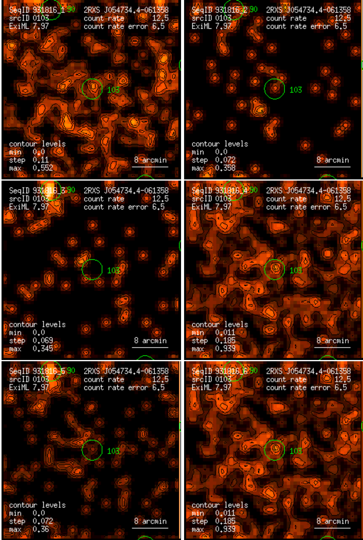
Figure 103: RASS 931816: detection 0103: band rate images, Gaussian filter: (1) PSPC channels 11 – 41, (2) 52 – 90, (3) 91 – 201, (4) 11 – 235, (5) 52 – 201, (6) 11 – 201. Broad band rates in counts/ks. Band rate contour levels in counts/ks/arcmin 2 .
