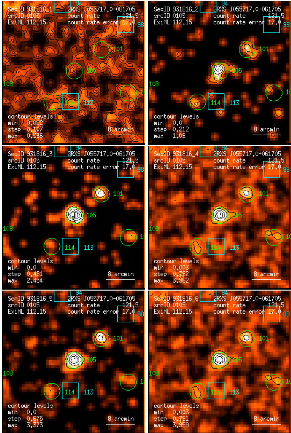
Figure 105: RASS 931816: detection 0105: band rate images, Gaussian filter: (1) PSPC channels 11 – 41, (2) 52 – 90, (3) 91 – 201, (4) 11 – 235, (5) 52 – 201, (6) 11 – 201. Broad band rates in counts/ks. Band rate contour levels in counts/ks/arcmin 2 .
