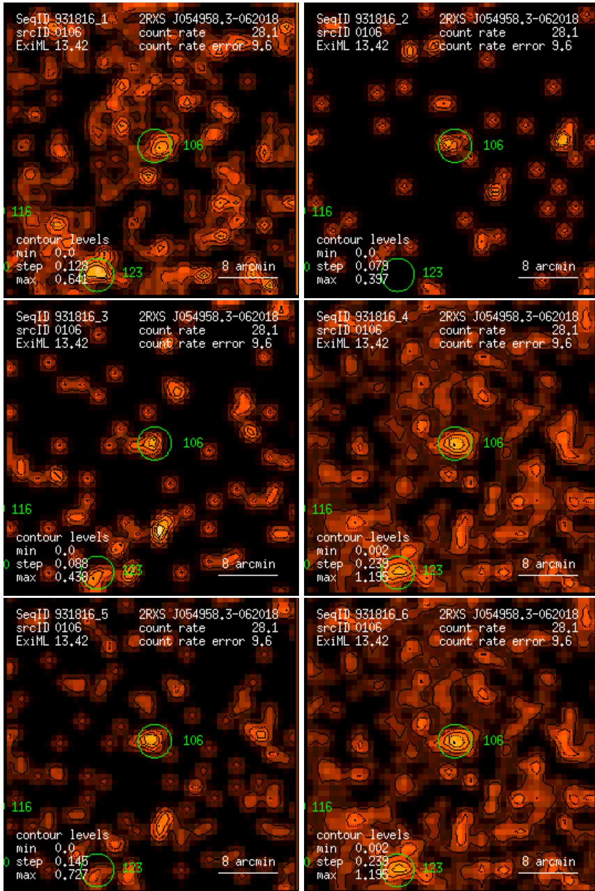
Figure 106: RASS 931816: detection 0106: band rate images, Gaussian filter: (1) PSPC channels 11 – 41, (2) 52 – 90, (3) 91 – 201, (4) 11 – 235, (5) 52 – 201, (6) 11 – 201. Broad band rates in counts/ks. Band rate contour levels in counts/ks/arcmin 2 .
