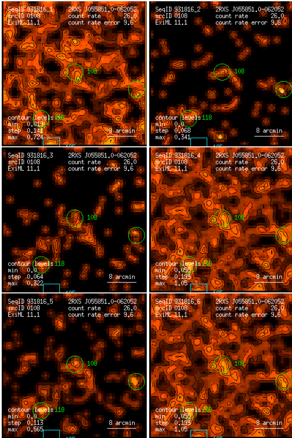
Figure 108: RASS 931816: detection 0108: band rate images, Gaussian filter: (1) PSPC channels 11 – 41, (2) 52 – 90, (3) 91 – 201, (4) 11 – 235, (5) 52 – 201, (6) 11 – 201. Broad band rates in counts/ks. Band rate contour levels in counts/ks/arcmin 2 .
