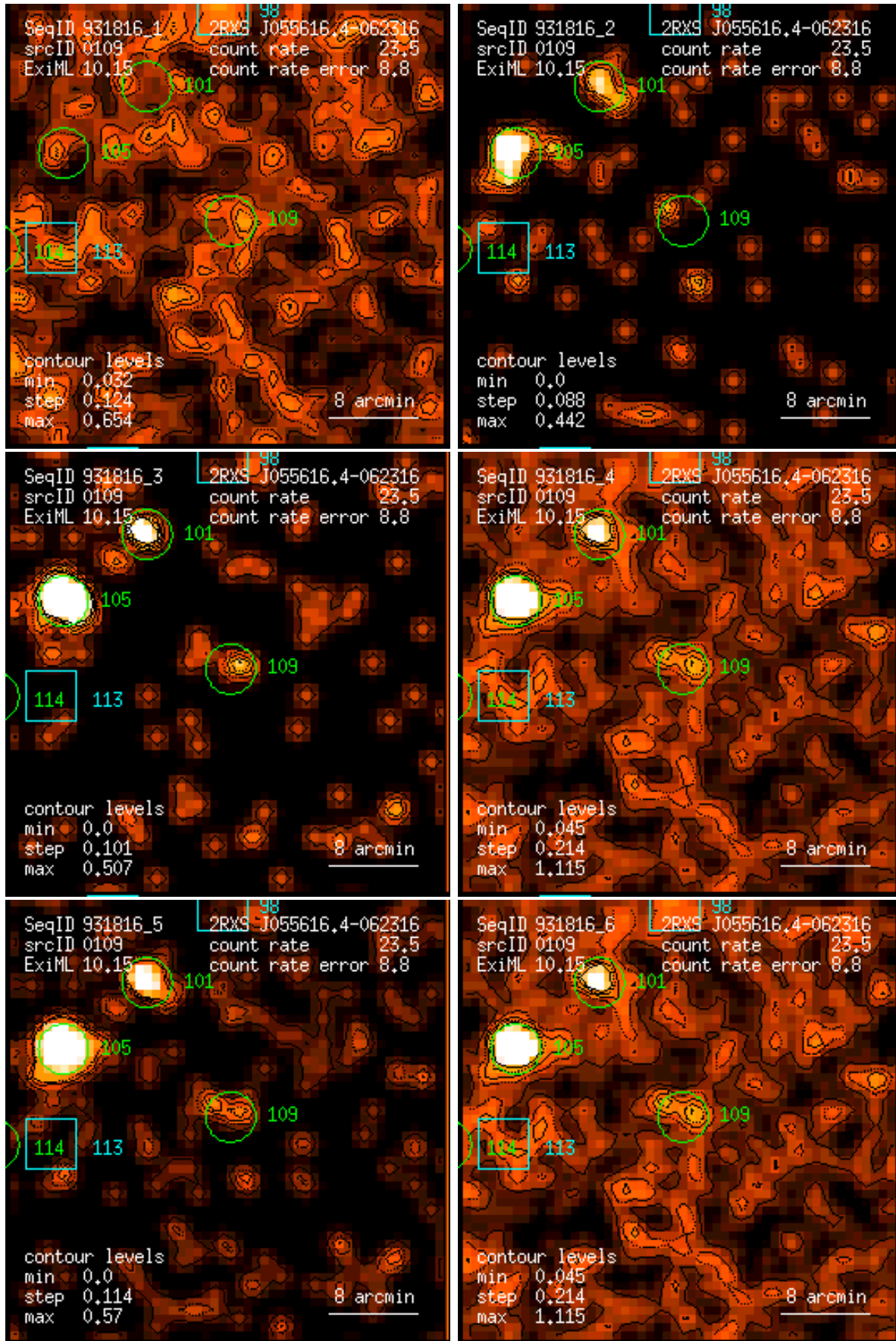
Figure 109: RASS 931816: detection 0109: band rate images, Gaussian filter: (1) PSPC channels 11 – 41, (2) 52 – 90, (3) 91 – 201, (4) 11 – 235, (5) 52 – 201, (6) 11 – 201. Broad band rates in counts/ks. Band rate contour levels in counts/ks/arcmin 2 .
