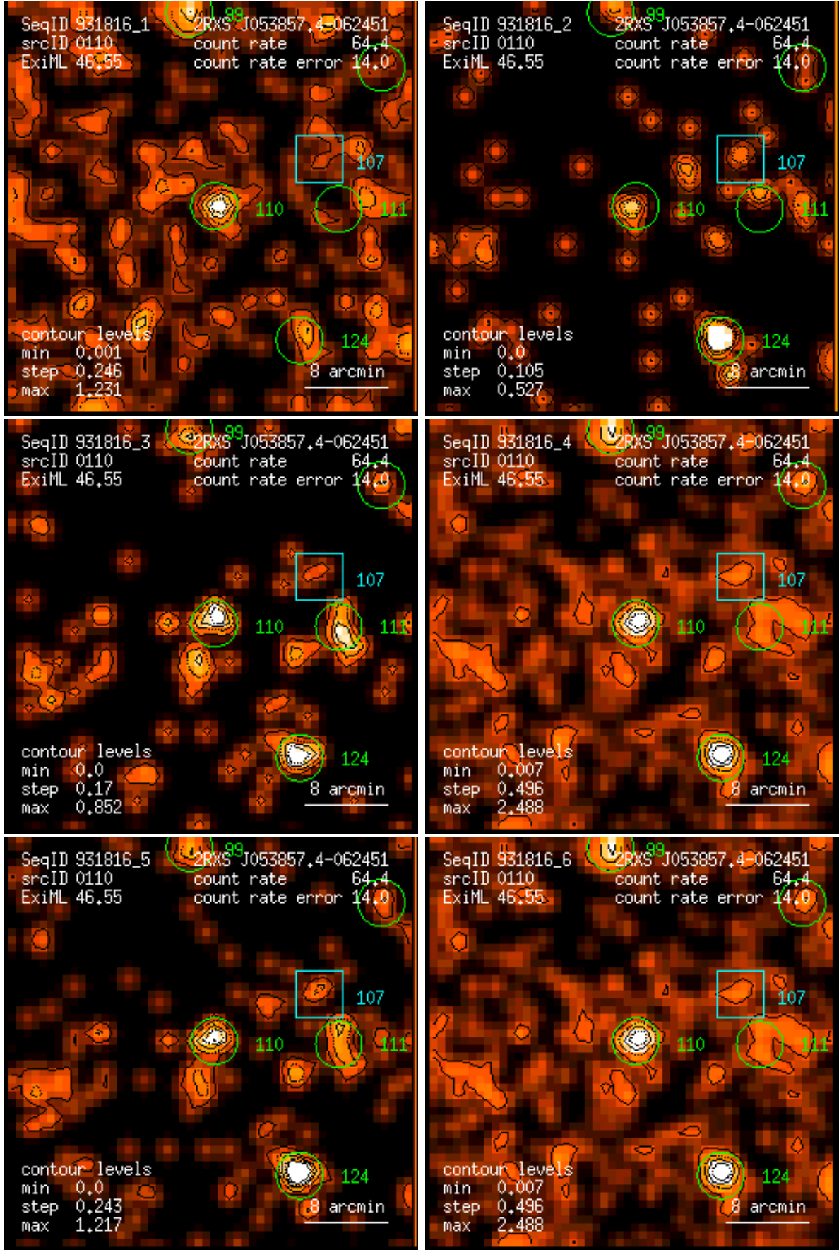
Figure 110: RASS 931816: detection 0110: band rate images, Gaussian filter: (1) PSPC channels 11 – 41, (2) 52 – 90, (3) 91 – 201, (4) 11 – 235, (5) 52 – 201, (6) 11 – 201. Broad band rates in counts/ks. Band rate contour levels in counts/ks/arcmin 2 .
