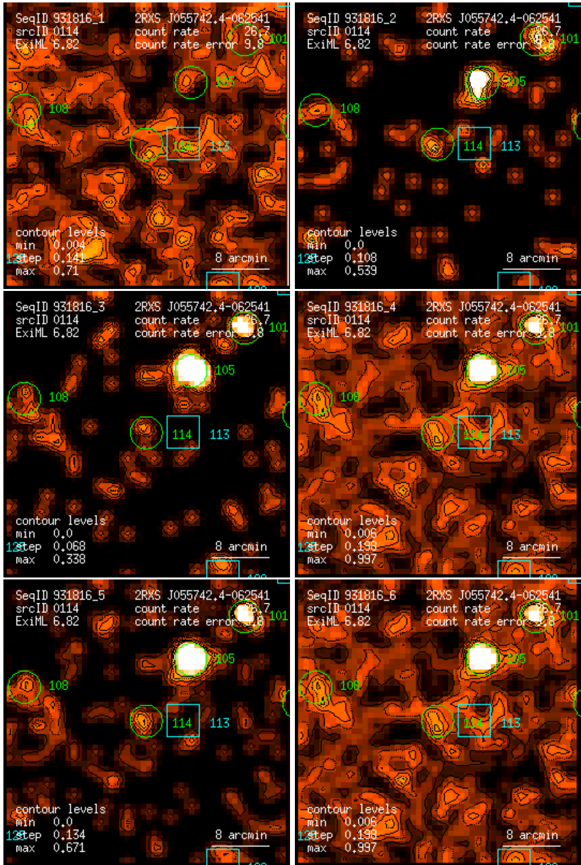
Figure 114: RASS 931816: detection 0114: band rate images, Gaussian filter: (1) PSPC channels 11 – 41, (2) 52 – 90, (3) 91 – 201, (4) 11 – 235, (5) 52 – 201, (6) 11 – 201. Broad band rates in counts/ks. Band rate contour levels in counts/ks/arcmin 2 .
