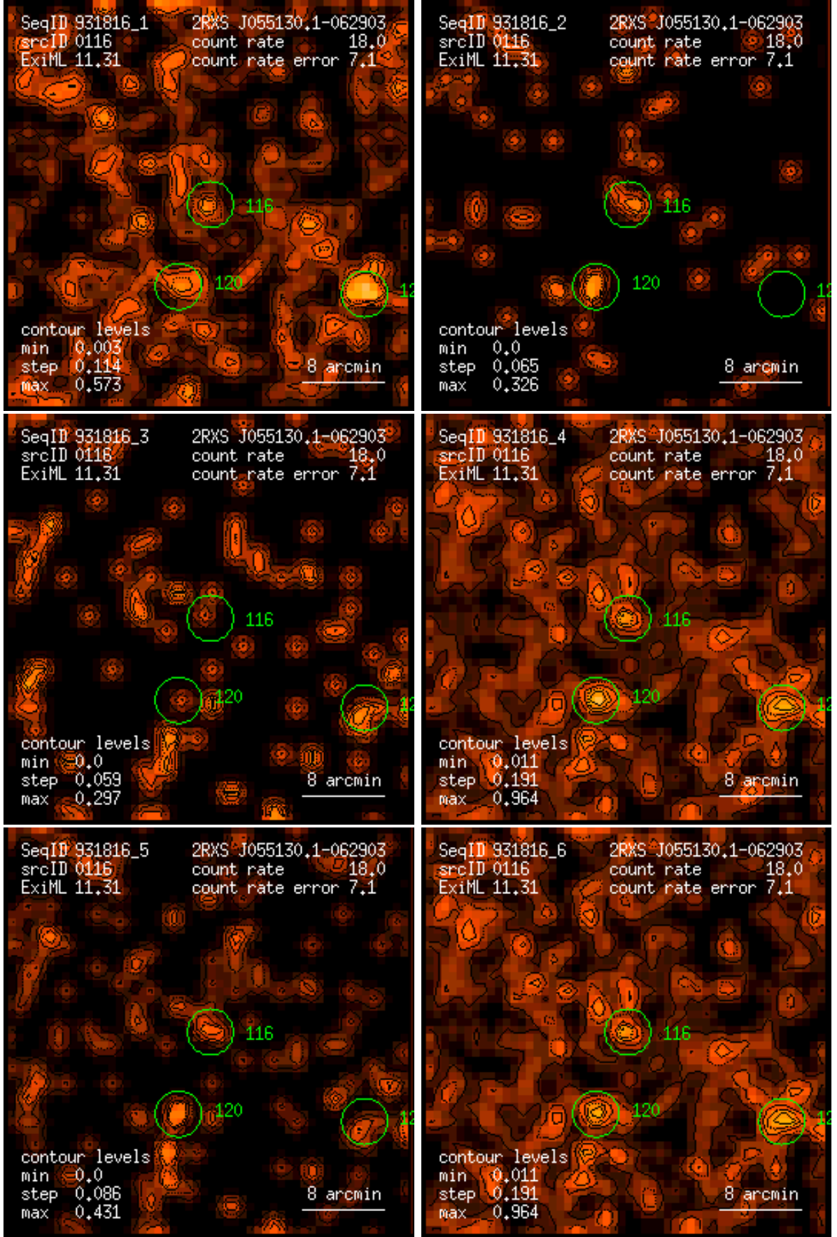
Figure 116: RASS 931816: detection 0116: band rate images, Gaussian filter: (1) PSPC channels 11 – 41, (2) 52 – 90, (3) 91 – 201, (4) 11 – 235, (5) 52 – 201, (6) 11 – 201. Broad band rates in counts/ks. Band rate contour levels in counts/ks/arcmin 2 .
