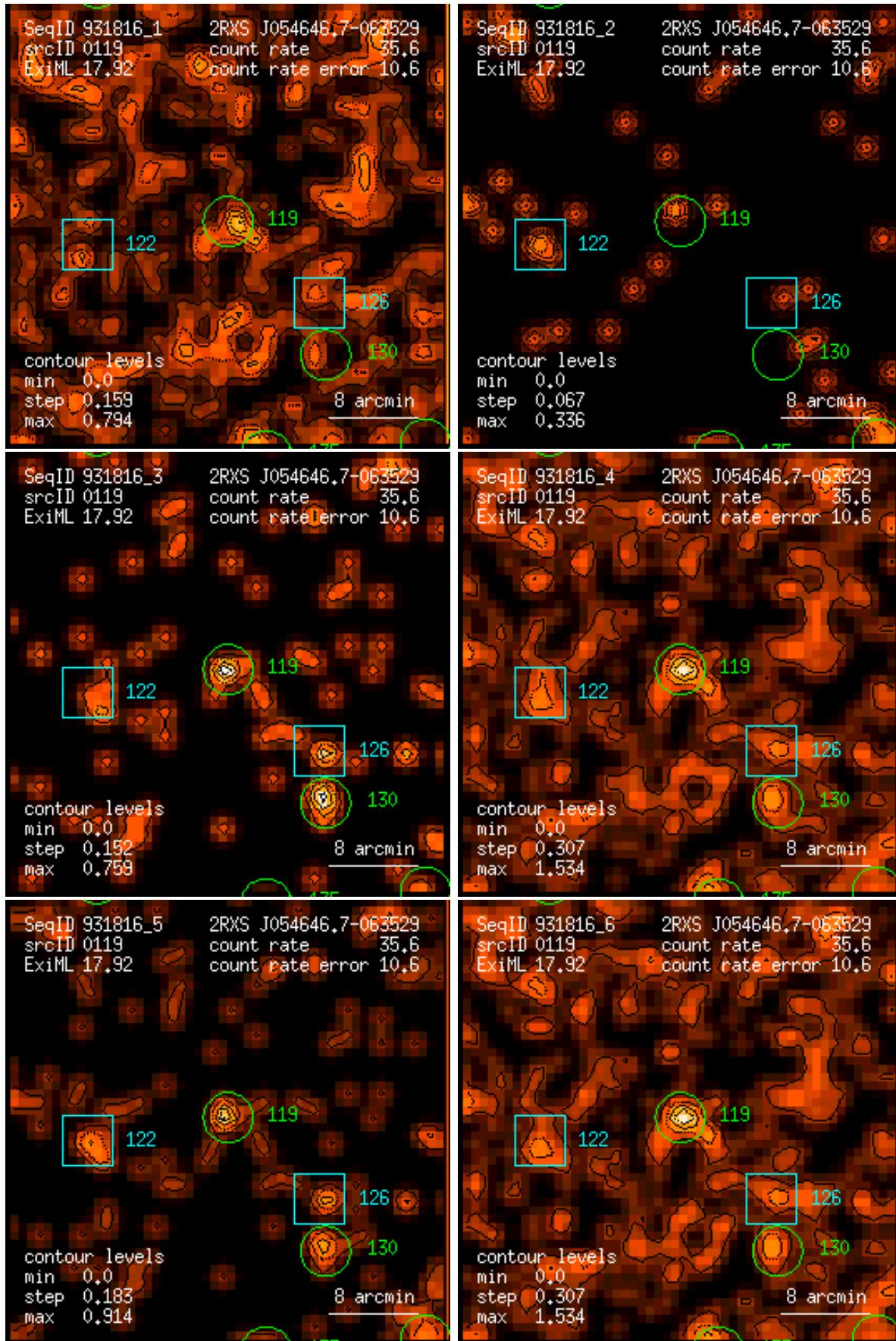
Figure 119: RASS 931816: detection 0119: band rate images, Gaussian filter: (1) PSPC channels 11 – 41, (2) 52 – 90, (3) 91 – 201, (4) 11 – 235, (5) 52 – 201, (6) 11 – 201. Broad band rates in counts/ks. Band rate contour levels in counts/ks/arcmin 2 .
