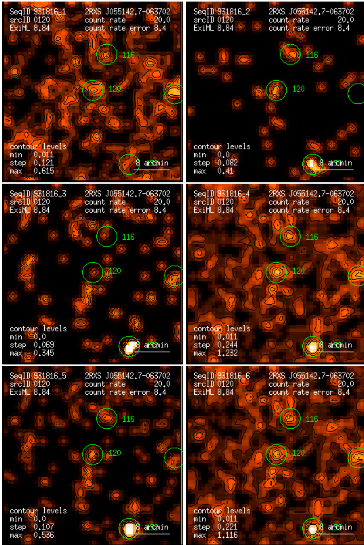
Figure 120: RASS 931816: detection 0120: band rate images, Gaussian filter: (1) PSPC channels 11 – 41, (2) 52 – 90, (3) 91 – 201, (4) 11 – 235, (5) 52 – 201, (6) 11 – 201. Broad band rates in counts/ks. Band rate contour levels in counts/ks/arcmin 2 .
