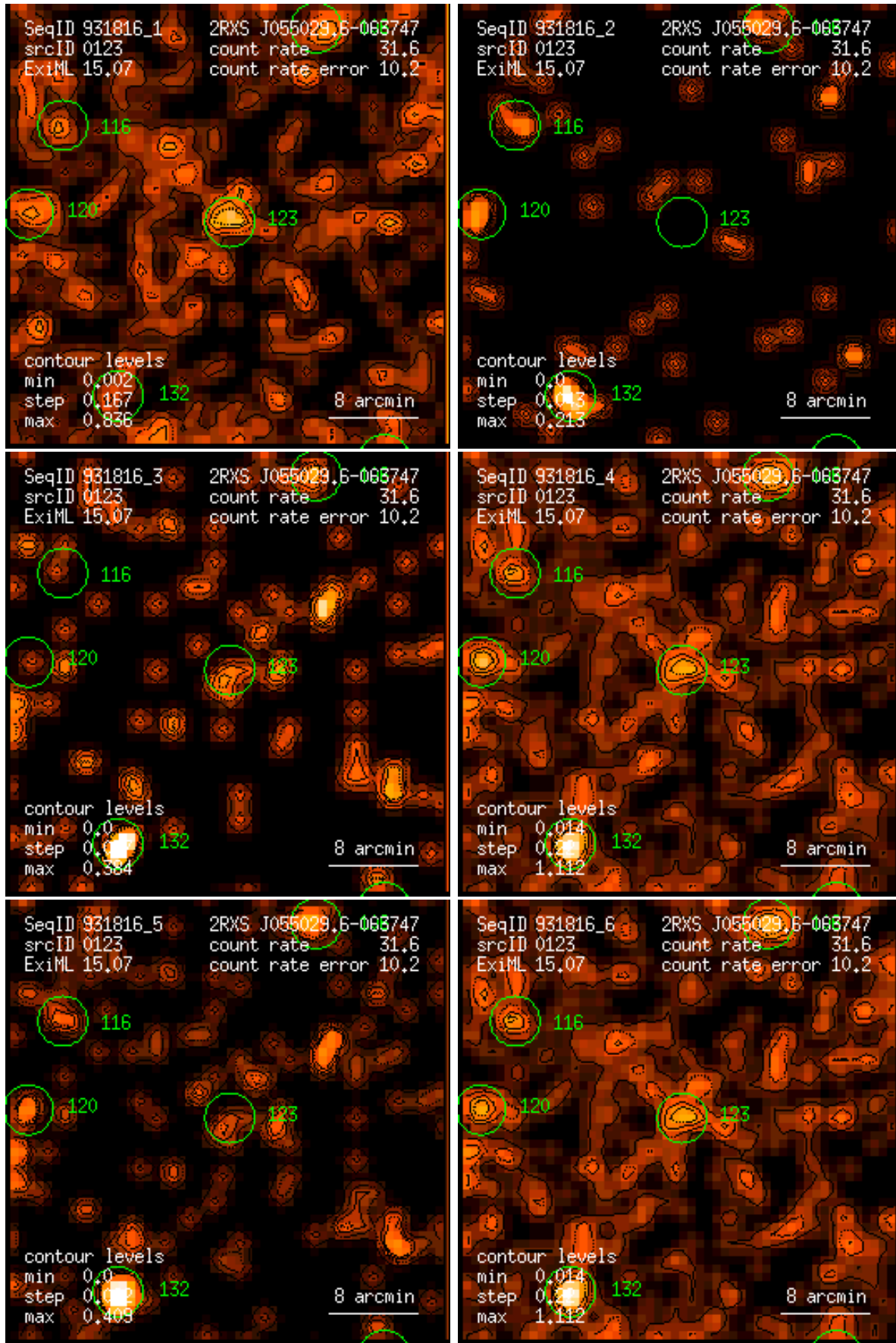
Figure 123: RASS 931816: detection 0123: band rate images, Gaussian filter: (1) PSPC channels 11 – 41, (2) 52 – 90, (3) 91 – 201, (4) 11 – 235, (5) 52 – 201, (6) 11 – 201. Broad band rates in counts/ks. Band rate contour levels in counts/ks/arcmin 2 .
