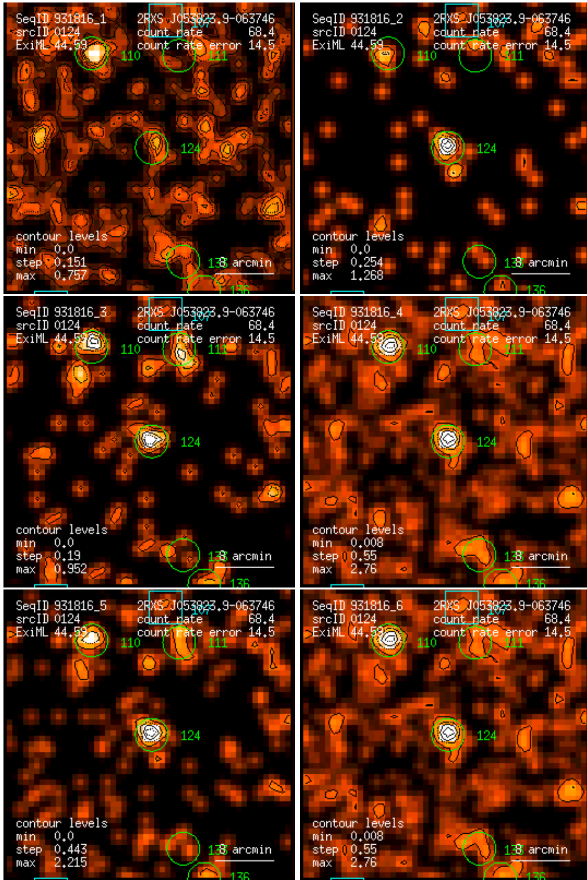
Figure 124: RASS 931816: detection 0124: band rate images, Gaussian filter: (1) PSPC channels 11 – 41, (2) 52 – 90, (3) 91 – 201, (4) 11 – 235, (5) 52 – 201, (6) 11 – 201. Broad band rates in counts/ks. Band rate contour levels in counts/ks/arcmin 2 .
