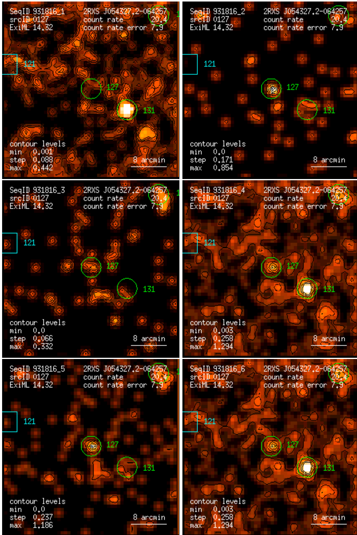
Figure 127: RASS 931816: detection 0127: band rate images, Gaussian filter: (1) PSPC channels 11 – 41, (2) 52 – 90, (3) 91 – 201, (4) 11 – 235, (5) 52 – 201, (6) 11 – 201. Broad band rates in counts/ks. Band rate contour levels in counts/ks/arcmin 2 .
