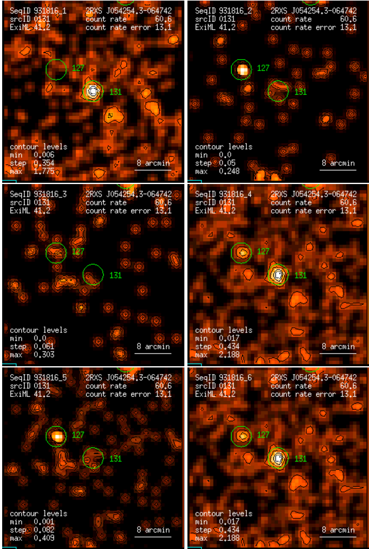
Figure 131: RASS 931816: detection 0131: band rate images, Gaussian filter: (1) PSPC channels 11 – 41, (2) 52 – 90, (3) 91 – 201, (4) 11 – 235, (5) 52 – 201, (6) 11 – 201. Broad band rates in counts/ks. Band rate contour levels in counts/ks/arcmin 2 .
