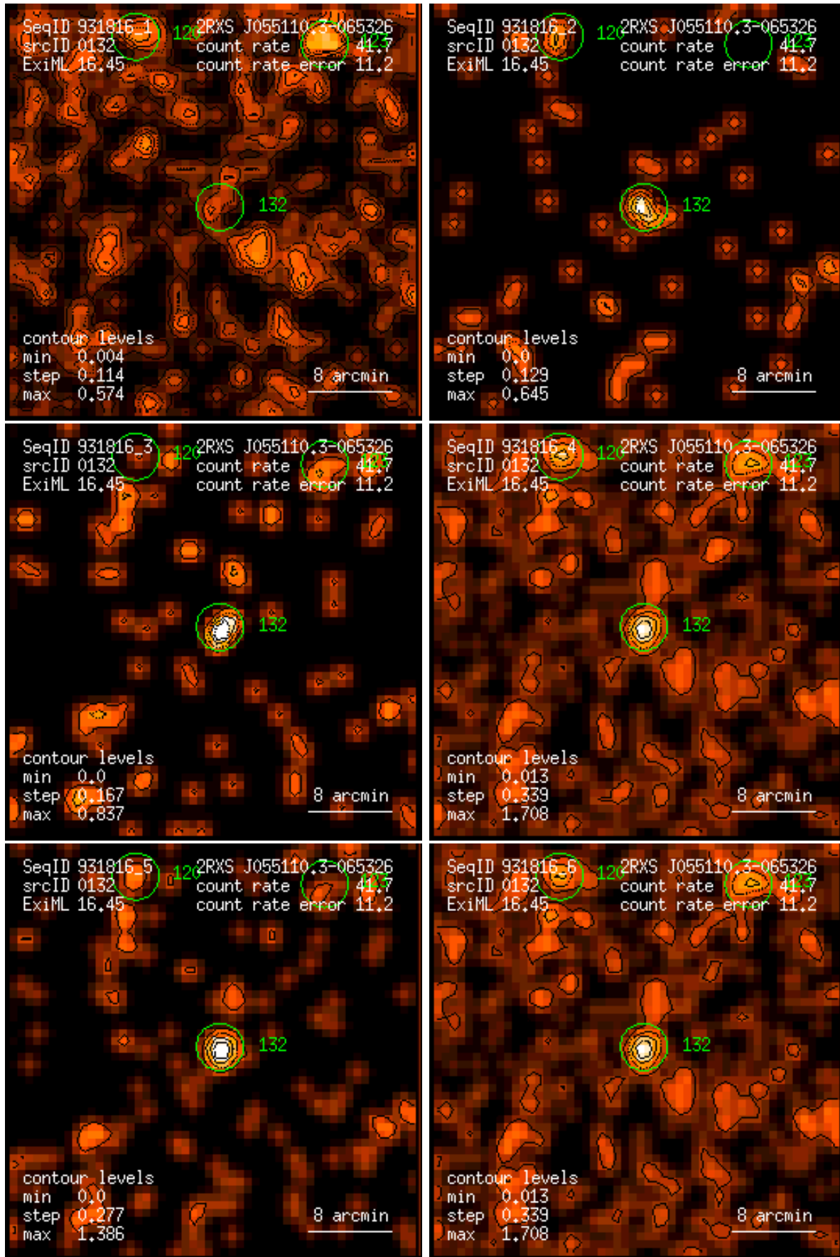
Figure 132: RASS 931816: detection 0132: band rate images, Gaussian filter: (1) PSPC channels 11 – 41, (2) 52 – 90, (3) 91 – 201, (4) 11 – 235, (5) 52 – 201, (6) 11 – 201. Broad band rates in counts/ks. Band rate contour levels in counts/ks/arcmin 2 .
