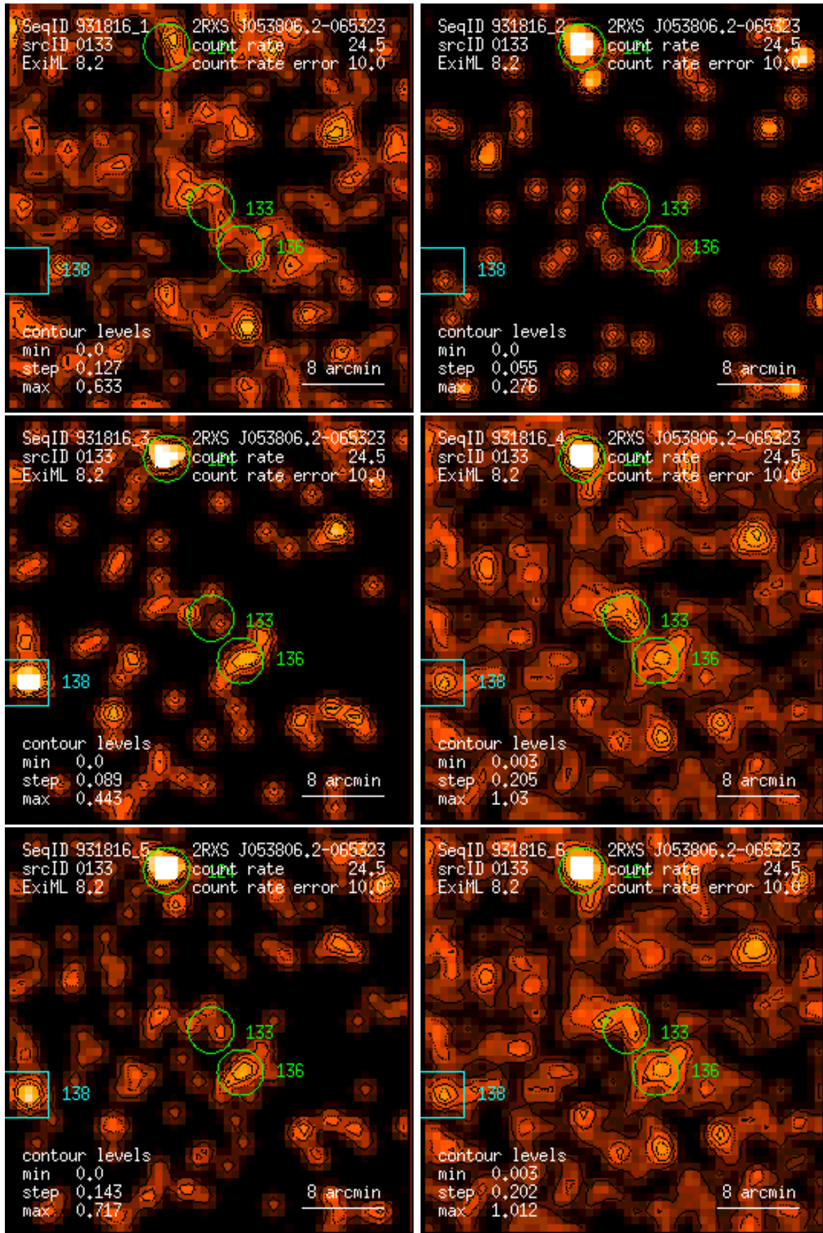
Figure 133: RASS 931816: detection 0133: band rate images, Gaussian filter: (1) PSPC channels 11 – 41, (2) 52 – 90, (3) 91 – 201, (4) 11 – 235, (5) 52 – 201, (6) 11 – 201. Broad band rates in counts/ks. Band rate contour levels in counts/ks/arcmin 2 .
