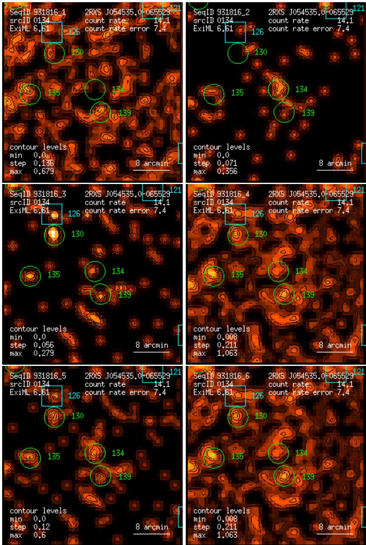
Figure 134: RASS 931816: detection 0134: band rate images, Gaussian filter: (1) PSPC channels 11 – 41, (2) 52 – 90, (3) 91 – 201, (4) 11 – 235, (5) 52 – 201, (6) 11 – 201. Broad band rates in counts/ks. Band rate contour levels in counts/ks/arcmin 2 .
