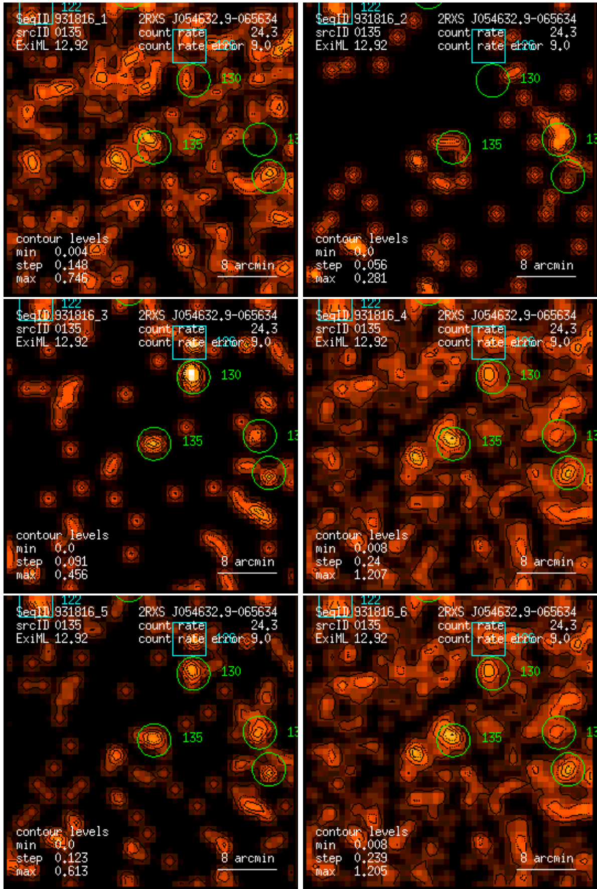
Figure 135: RASS 931816: detection 0135: band rate images, Gaussian filter: (1) PSPC channels 11 – 41, (2) 52 – 90, (3) 91 – 201, (4) 11 – 235, (5) 52 – 201, (6) 11 – 201. Broad band rates in counts/ks. Band rate contour levels in counts/ks/arcmin 2 .
