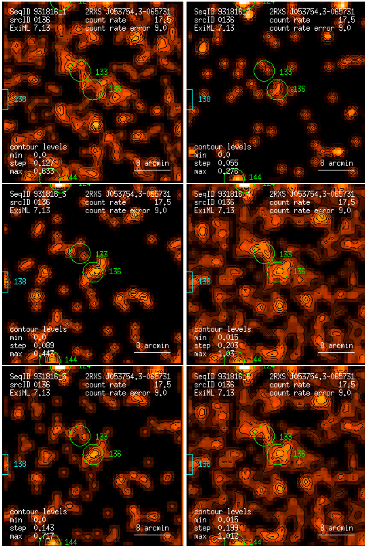
Figure 136: RASS 931816: detection 0136: band rate images, Gaussian filter: (1) PSPC channels 11 – 41, (2) 52 – 90, (3) 91 – 201, (4) 11 – 235, (5) 52 – 201, (6) 11 – 201. Broad band rates in counts/ks. Band rate contour levels in counts/ks/arcmin 2 .
