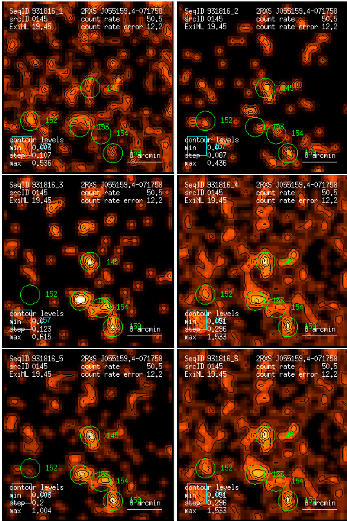
Figure 145: RASS 931816: detection 0145: band rate images, Gaussian filter: (1) PSPC channels 11 – 41, (2) 52 – 90, (3) 91 – 201, (4) 11 – 235, (5) 52 – 201, (6) 11 – 201. Broad band rates in counts/ks. Band rate contour levels in counts/ks/arcmin 2 .
