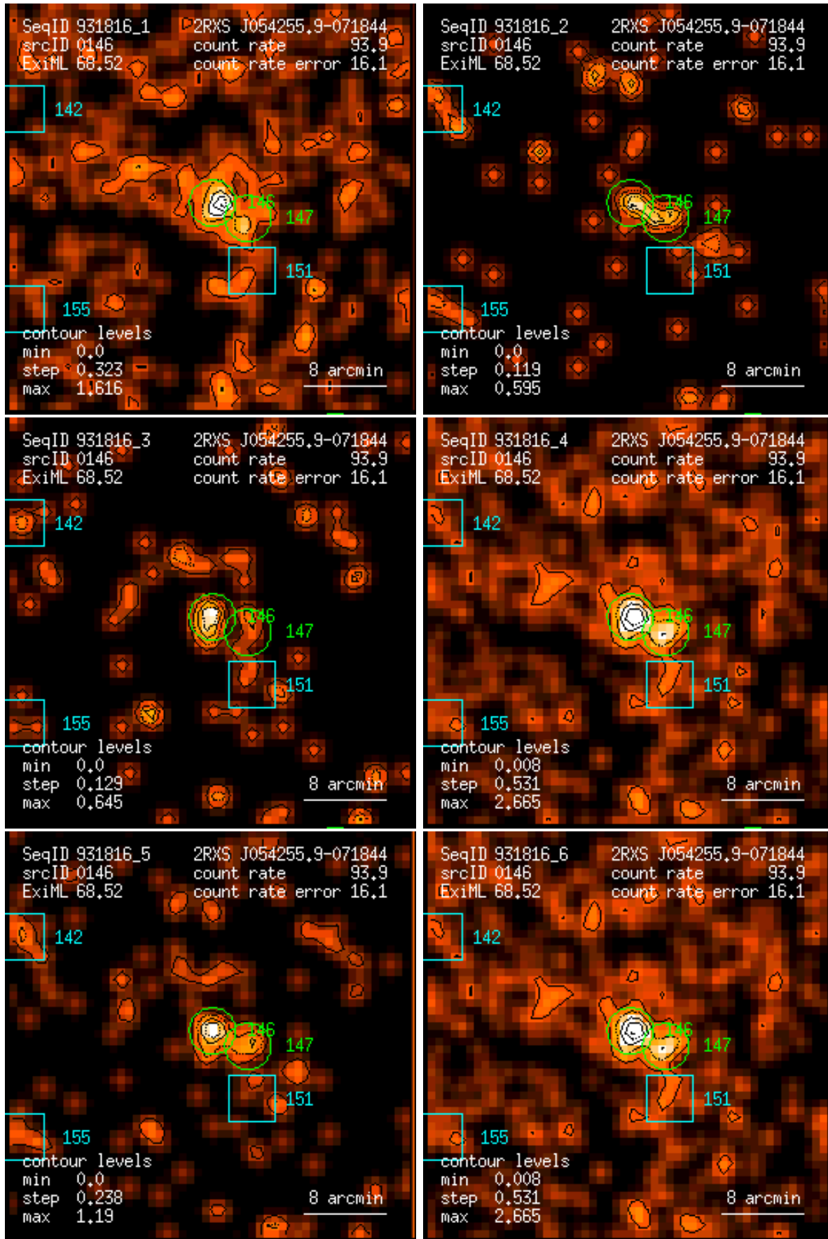
Figure 146: RASS 931816: detection 0146: band rate images, Gaussian filter: (1) PSPC channels 11 – 41, (2) 52 – 90, (3) 91 – 201, (4) 11 – 235, (5) 52 – 201, (6) 11 – 201. Broad band rates in counts/ks. Band rate contour levels in counts/ks/arcmin 2 .
