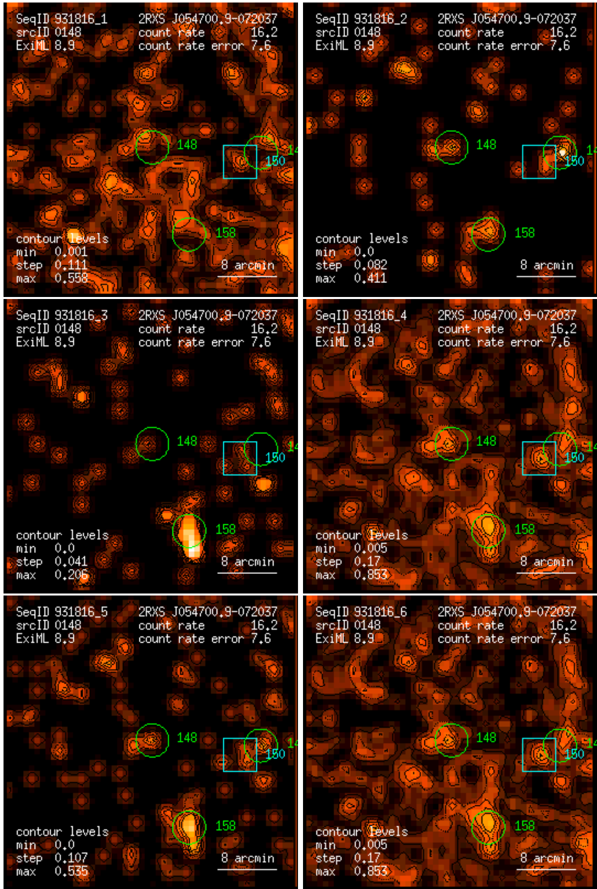
Figure 148: RASS 931816: detection 0148: band rate images, Gaussian filter: (1) PSPC channels 11 – 41, (2) 52 – 90, (3) 91 – 201, (4) 11 – 235, (5) 52 – 201, (6) 11 – 201. Broad band rates in counts/ks. Band rate contour levels in counts/ks/arcmin 2 .
