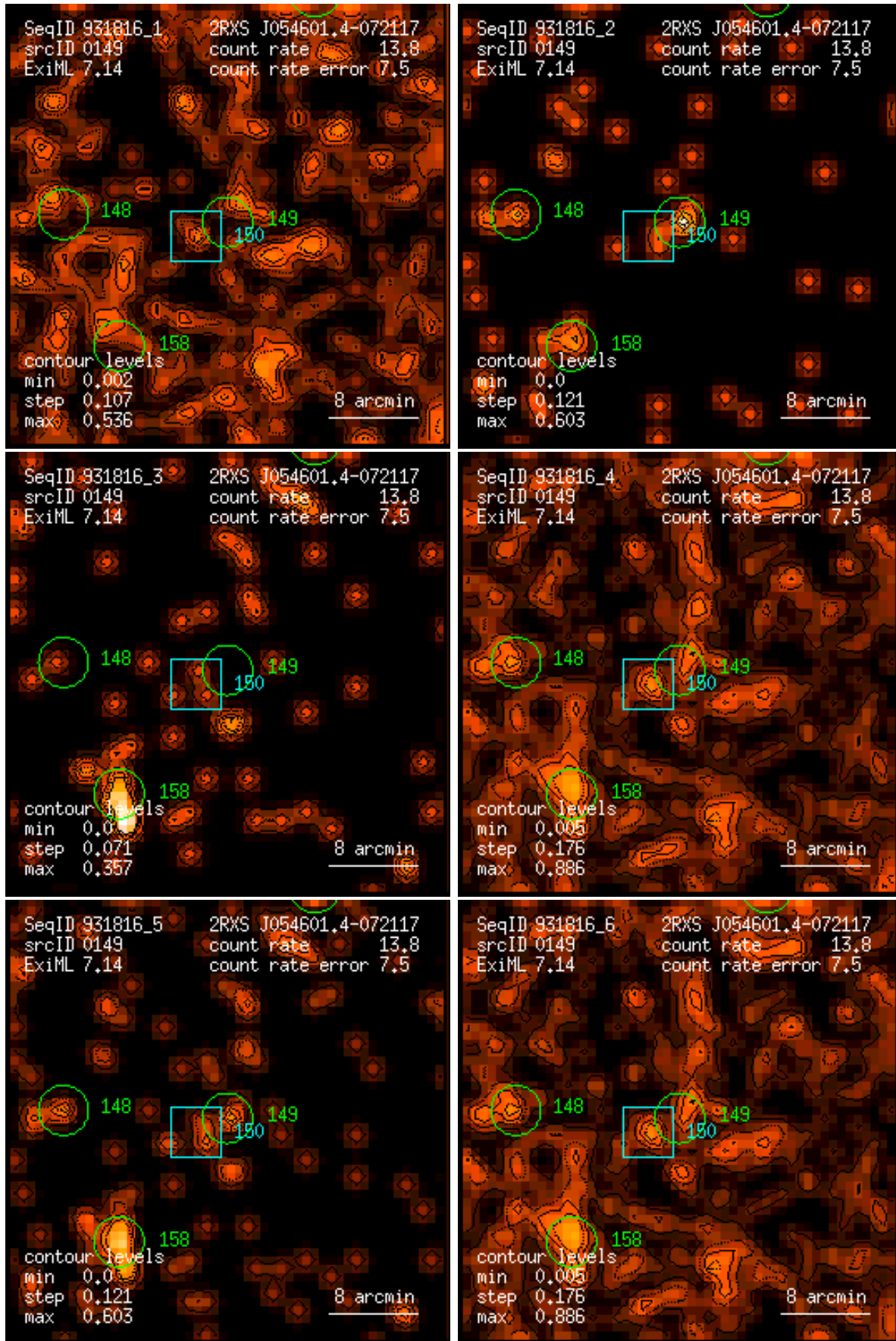
Figure 149: RASS 931816: detection 0149: band rate images, Gaussian filter: (1) PSPC channels 11 – 41, (2) 52 – 90, (3) 91 – 201, (4) 11 – 235, (5) 52 – 201, (6) 11 – 201. Broad band rates in counts/ks. Band rate contour levels in counts/ks/arcmin 2 .
