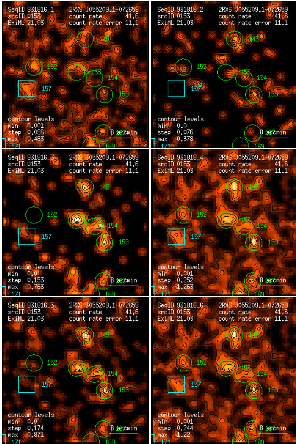
Figure 153: RASS 931816: detection 0153: band rate images, Gaussian filter: (1) PSPC channels 11 – 41, (2) 52 – 90, (3) 91 – 201, (4) 11 – 235, (5) 52 – 201, (6) 11 – 201. Broad band rates in counts/ks. Band rate contour levels in counts/ks/arcmin 2 .
