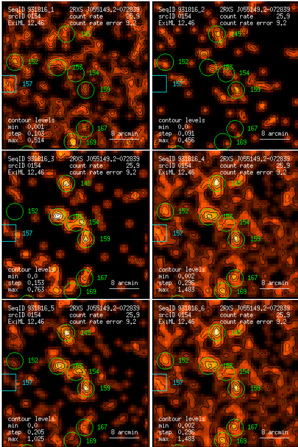
Figure 154: RASS 931816: detection 0154: band rate images, Gaussian filter: (1) PSPC channels 11 – 41, (2) 52 – 90, (3) 91 – 201, (4) 11 – 235, (5) 52 – 201, (6) 11 – 201. Broad band rates in counts/ks. Band rate contour levels in counts/ks/arcmin 2 .
