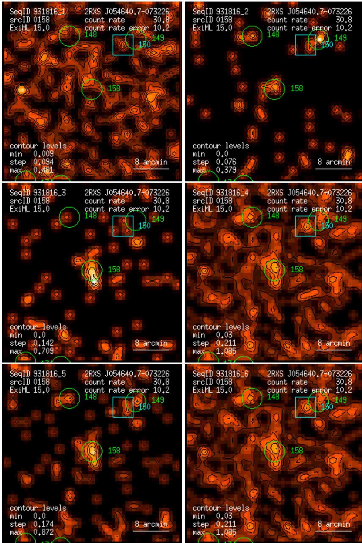
Figure 158: RASS 931816: detection 0158: band rate images, Gaussian filter: (1) PSPC channels 11 – 41, (2) 52 – 90, (3) 91 – 201, (4) 11 – 235, (5) 52 – 201, (6) 11 – 201. Broad band rates in counts/ks. Band rate contour levels in counts/ks/arcmin 2 .
