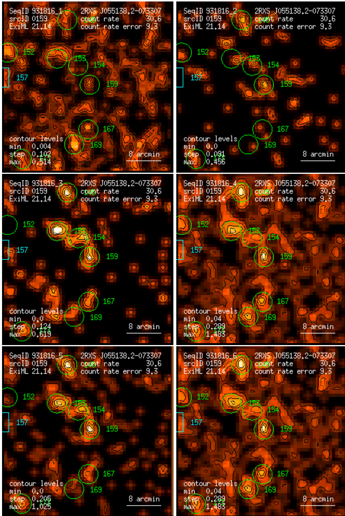
Figure 159: RASS 931816: detection 0159: band rate images, Gaussian filter: (1) PSPC channels 11 – 41, (2) 52 – 90, (3) 91 – 201, (4) 11 – 235, (5) 52 – 201, (6) 11 – 201. Broad band rates in counts/ks. Band rate contour levels in counts/ks/arcmin 2 .
