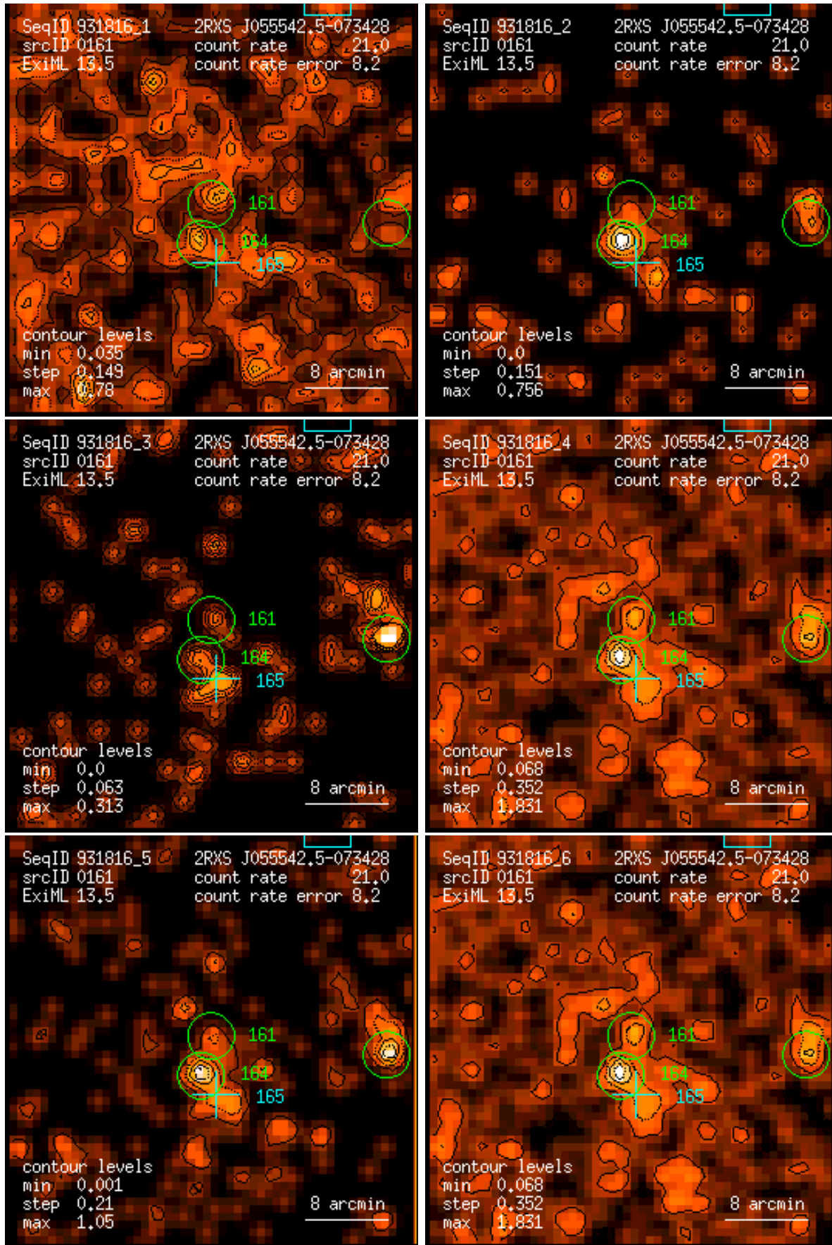
Figure 161: RASS 931816: detection 0161: band rate images, Gaussian filter: (1) PSPC channels 11 – 41, (2) 52 – 90, (3) 91 – 201, (4) 11 – 235, (5) 52 – 201, (6) 11 – 201. Broad band rates in counts/ks. Band rate contour levels in counts/ks/arcmin 2 .
