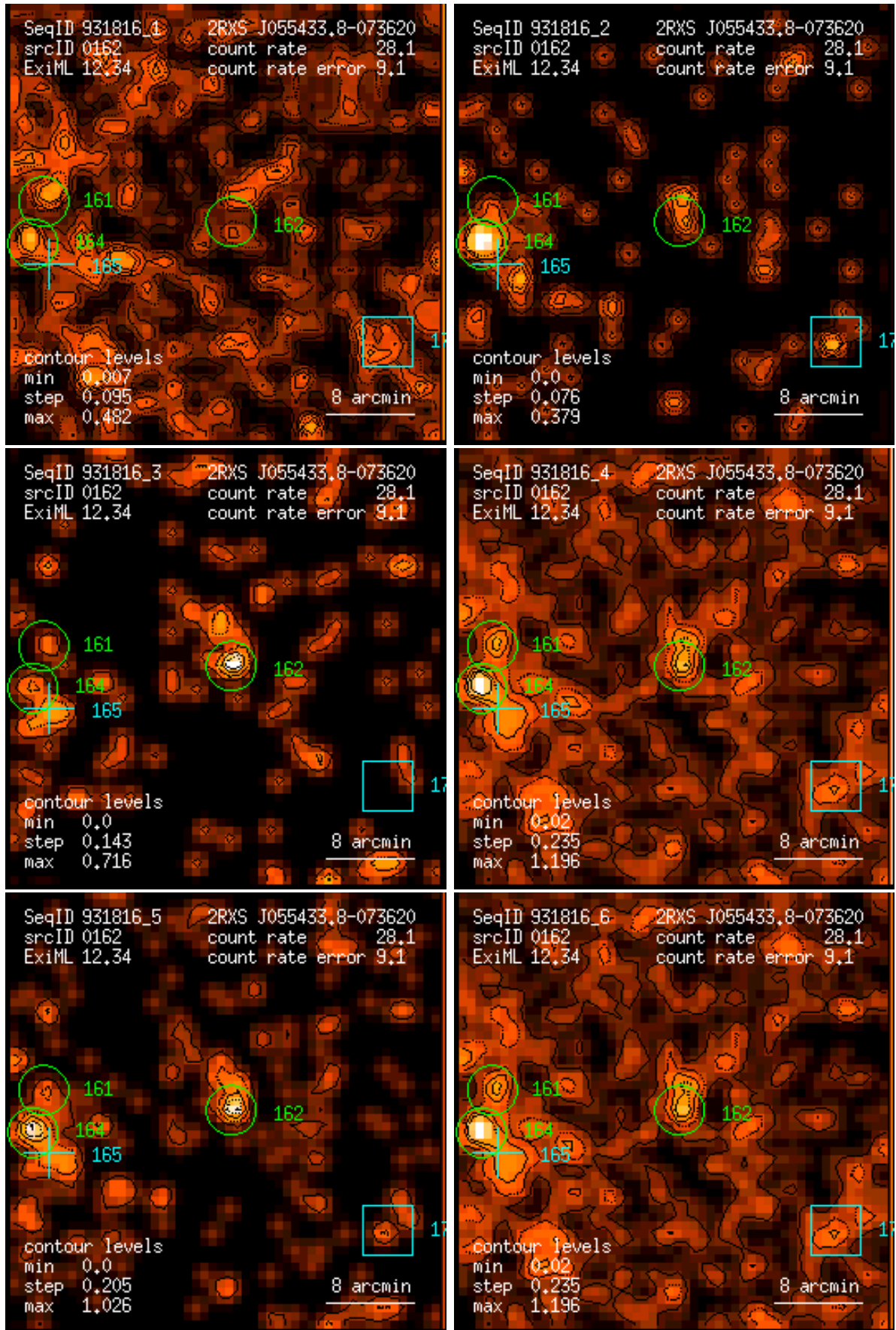
Figure 162: RASS 931816: detection 0162: band rate images, Gaussian filter: (1) PSPC channels 11 – 41, (2) 52 – 90, (3) 91 – 201, (4) 11 – 235, (5) 52 – 201, (6) 11 – 201. Broad band rates in counts/ks. Band rate contour levels in counts/ks/arcmin 2 .
