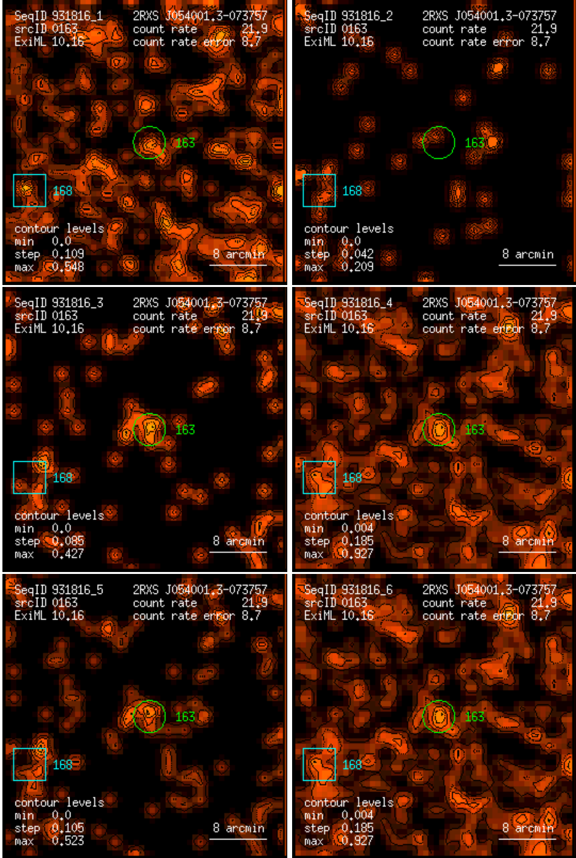
Figure 163: RASS 931816: detection 0163: band rate images, Gaussian filter: (1) PSPC channels 11 – 41, (2) 52 – 90, (3) 91 – 201, (4) 11 – 235, (5) 52 – 201, (6) 11 – 201. Broad band rates in counts/ks. Band rate contour levels in counts/ks/arcmin 2 .
