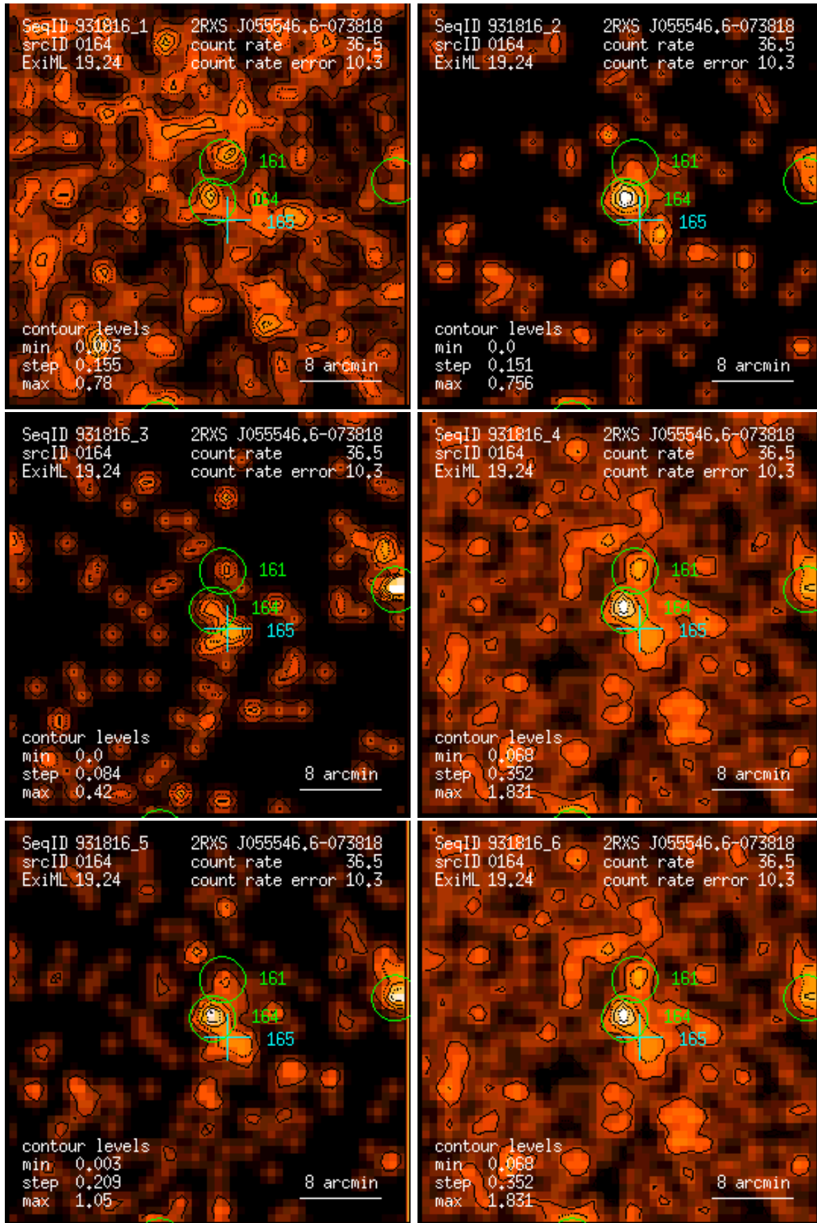
Figure 164: RASS 931816: detection 0164: band rate images, Gaussian filter: (1) PSPC channels 11 – 41, (2) 52 – 90, (3) 91 – 201, (4) 11 – 235, (5) 52 – 201, (6) 11 – 201. Broad band rates in counts/ks. Band rate contour levels in counts/ks/arcmin 2 .
