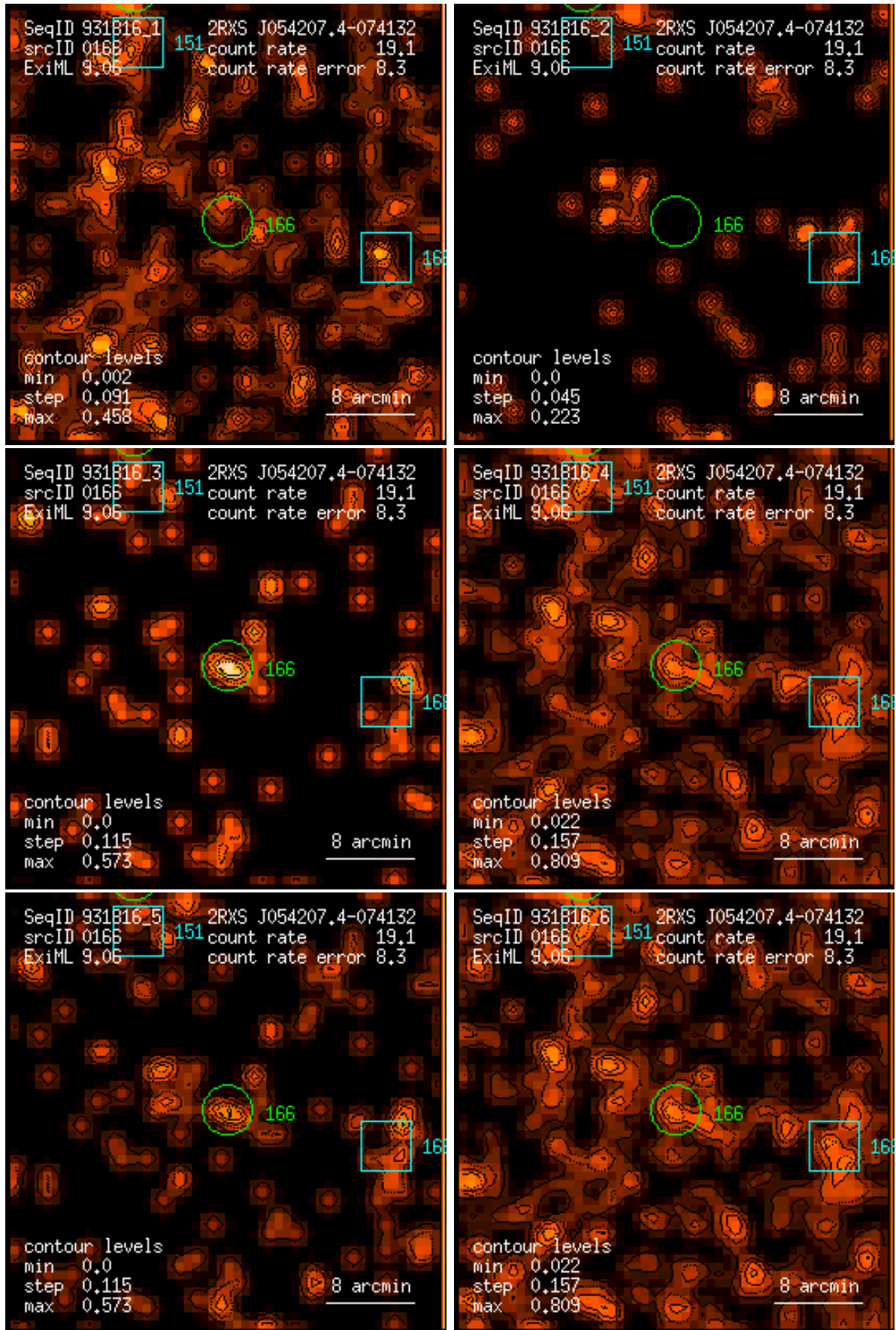
Figure 166: RASS 931816: detection 0166: band rate images, Gaussian filter: (1) PSPC channels 11 – 41, (2) 52 – 90, (3) 91 – 201, (4) 11 – 235, (5) 52 – 201, (6) 11 – 201. Broad band rates in counts/ks. Band rate contour levels in counts/ks/arcmin 2 .
