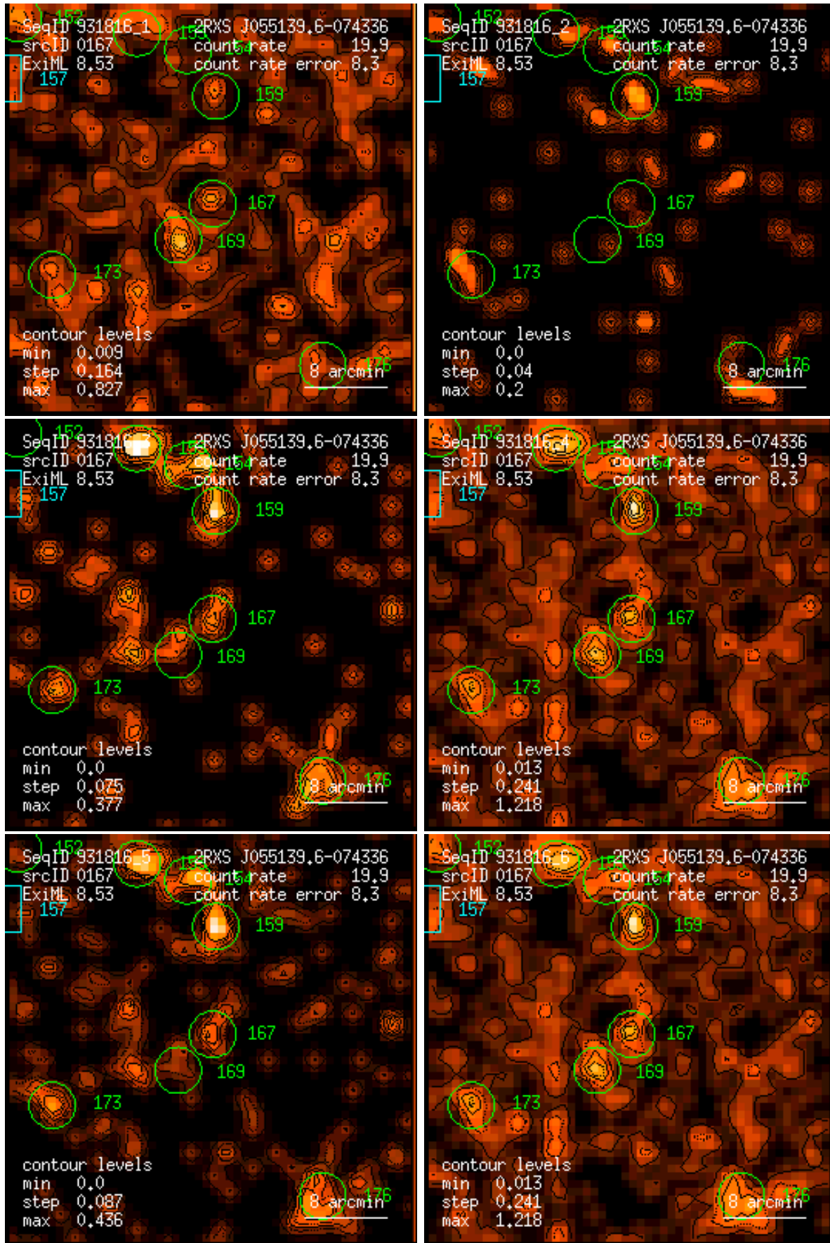
Figure 167: RASS 931816: detection 0167: band rate images, Gaussian filter: (1) PSPC channels 11 – 41, (2) 52 – 90, (3) 91 – 201, (4) 11 – 235, (5) 52 – 201, (6) 11 – 201. Broad band rates in counts/ks. Band rate contour levels in counts/ks/arcmin 2 .
