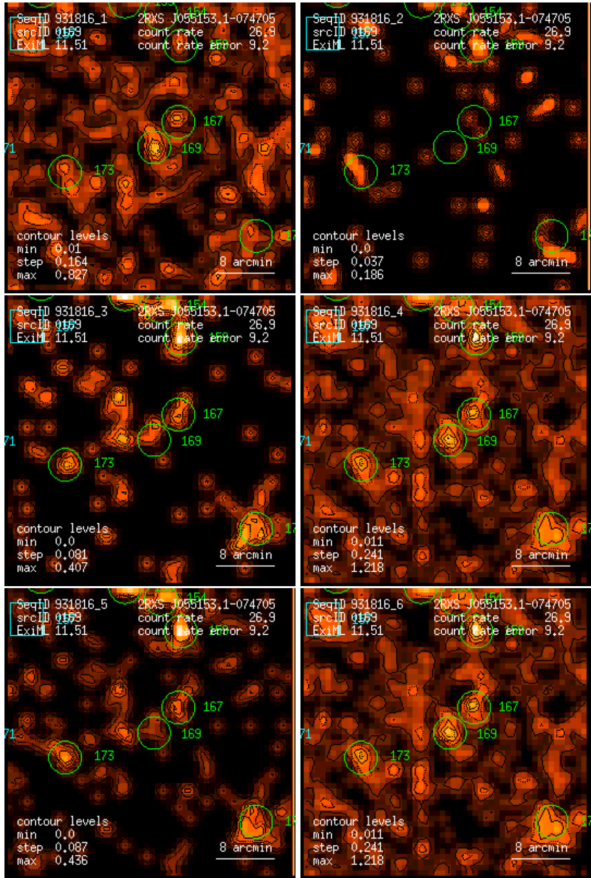
Figure 169: RASS 931816: detection 0169: band rate images, Gaussian filter: (1) PSPC channels 11 – 41, (2) 52 – 90, (3) 91 – 201, (4) 11 – 235, (5) 52 – 201, (6) 11 – 201. Broad band rates in counts/ks. Band rate contour levels in counts/ks/arcmin 2 .
