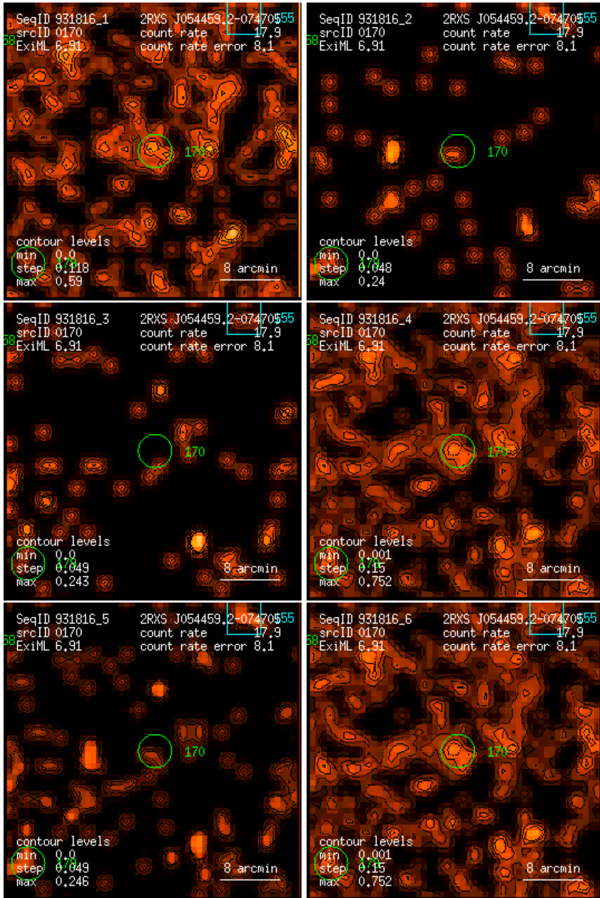
Figure 170: RASS 931816: detection 0170: band rate images, Gaussian filter: (1) PSPC channels 11 – 41, (2) 52 – 90, (3) 91 – 201, (4) 11 – 235, (5) 52 – 201, (6) 11 – 201. Broad band rates in counts/ks. Band rate contour levels in counts/ks/arcmin 2 .
