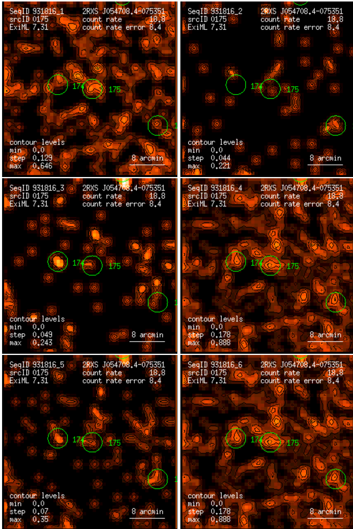
Figure 175: RASS 931816: detection 0175: band rate images, Gaussian filter: (1) PSPC channels 11 – 41, (2) 52 – 90, (3) 91 – 201, (4) 11 – 235, (5) 52 – 201, (6) 11 – 201. Broad band rates in counts/ks. Band rate contour levels in counts/ks/arcmin 2 .
