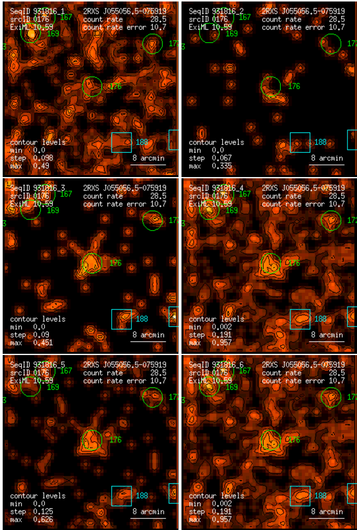
Figure 176: RASS 931816: detection 0176: band rate images, Gaussian filter: (1) PSPC channels 11 – 41, (2) 52 – 90, (3) 91 – 201, (4) 11 – 235, (5) 52 – 201, (6) 11 – 201. Broad band rates in counts/ks. Band rate contour levels in counts/ks/arcmin 2 .
