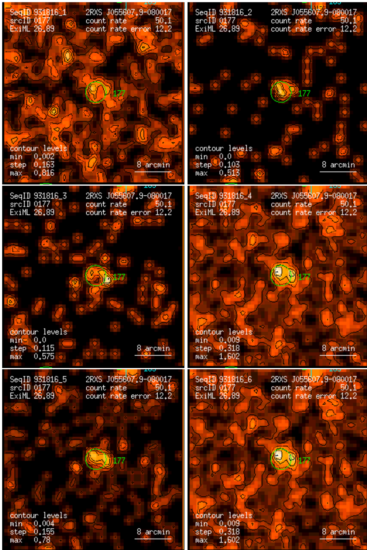
Figure 177: RASS 931816: detection 0177: band rate images, Gaussian filter: (1) PSPC channels 11 – 41, (2) 52 – 90, (3) 91 – 201, (4) 11 – 235, (5) 52 – 201, (6) 11 – 201. Broad band rates in counts/ks. Band rate contour levels in counts/ks/arcmin 2 .
