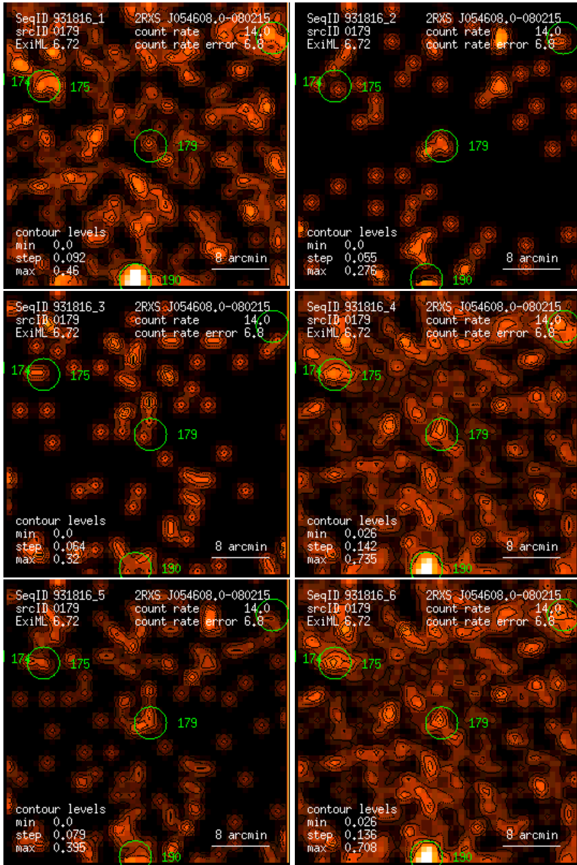
Figure 179: RASS 931816: detection 0179: band rate images, Gaussian filter: (1) PSPC channels 11 – 41, (2) 52 – 90, (3) 91 – 201, (4) 11 – 235, (5) 52 – 201, (6) 11 – 201. Broad band rates in counts/ks. Band rate contour levels in counts/ks/arcmin 2 .
