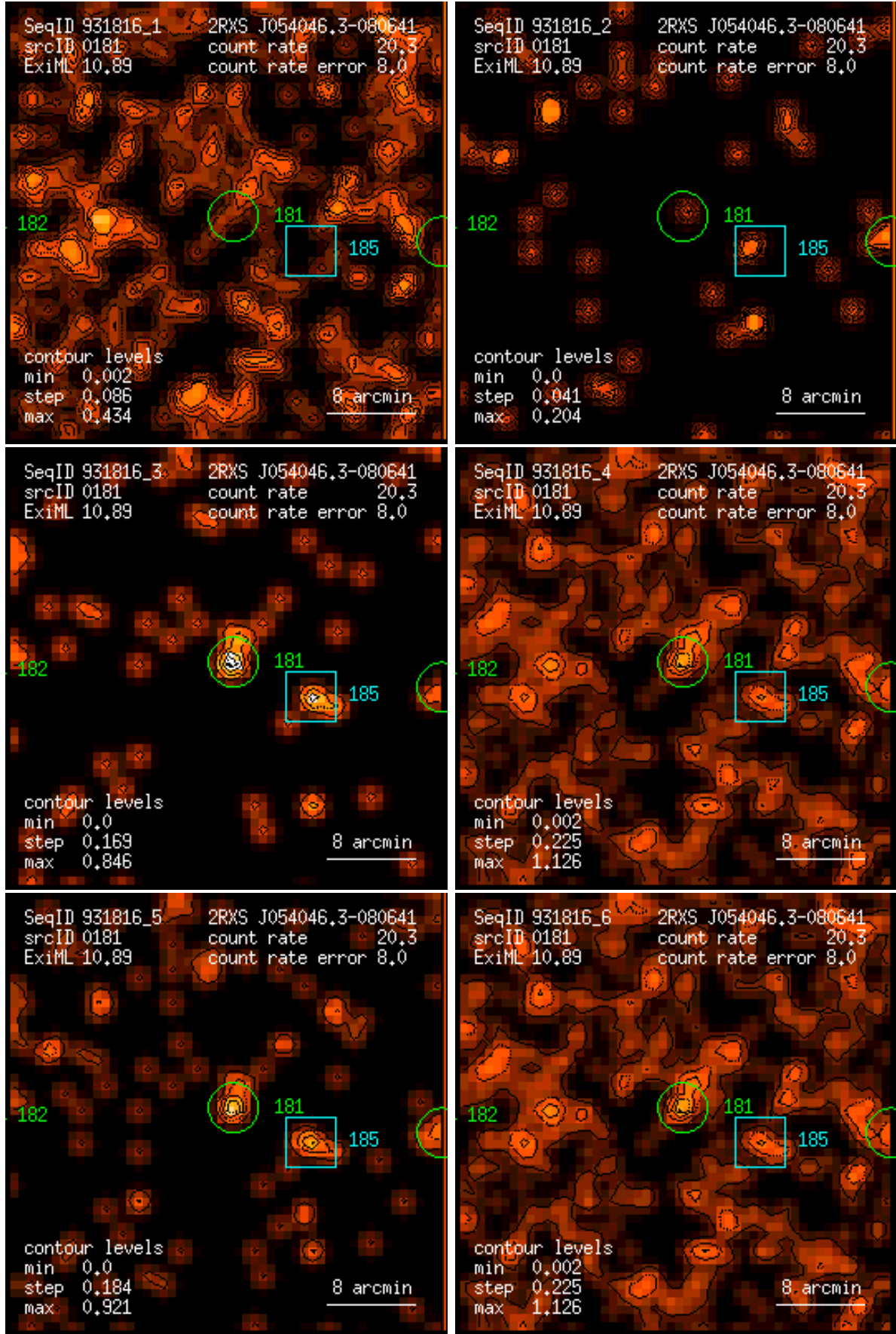
Figure 181: RASS 931816: detection 0181: band rate images, Gaussian filter: (1) PSPC channels 11 – 41, (2) 52 – 90, (3) 91 – 201, (4) 11 – 235, (5) 52 – 201, (6) 11 – 201. Broad band rates in counts/ks. Band rate contour levels in counts/ks/arcmin 2 .
