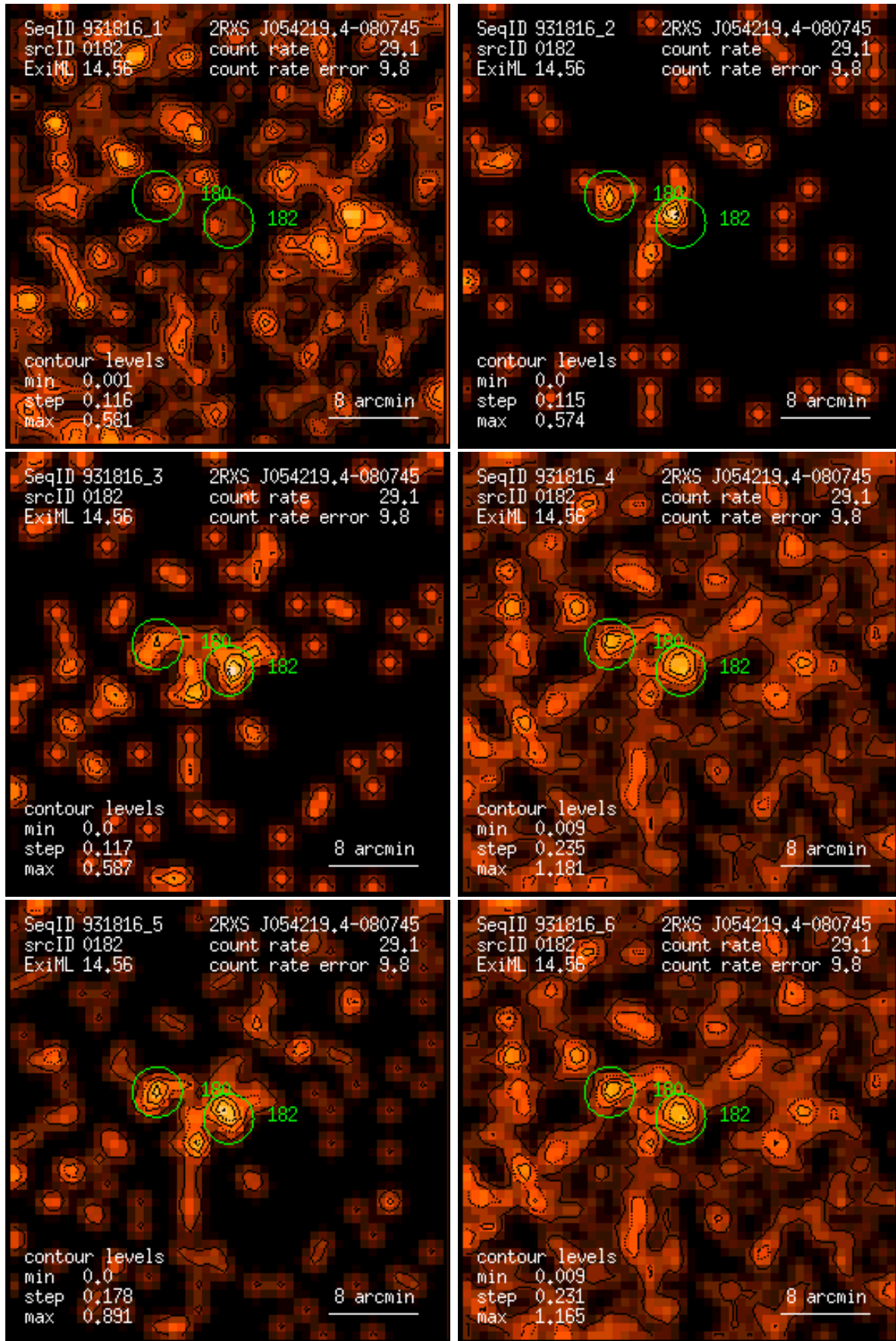
Figure 182: RASS 931816: detection 0182: band rate images, Gaussian filter: (1) PSPC channels 11 – 41, (2) 52 – 90, (3) 91 – 201, (4) 11 – 235, (5) 52 – 201, (6) 11 – 201. Broad band rates in counts/ks. Band rate contour levels in counts/ks/arcmin 2 .
